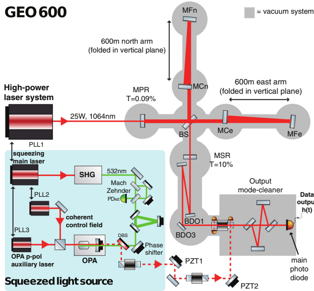
FIG. 1. The layout of the squeezing application to the GEO 600 detector. The three Faraday isolators used for squeezed light injection are depicted. The squeezed light is injected such that it overlaps the main beam with the correct polarization at the MSR. The photodiodes shown at the in-vacuum Faraday isolator are used for polarization diagnostics.
