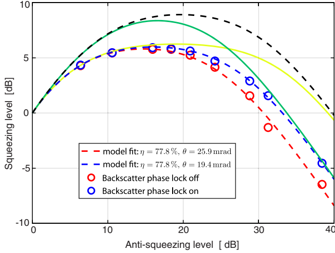
FIG. 3. Detected squeezing level as a function of measured antisqueezing measured at 5.2 kHz. The blue and red traces represent fits to the respective data points. The fitting procedure fits a common parameter for optical efficiency, \eta . The two solid traces represent estimates of the detectable squeezing level if a factor of 2 reduction of optical loss (green) and phase noise (yellow) could be realized. The dashed black trace is a factor of 2 improvement in both. This shows that we are still primarily limited by optical loss.
