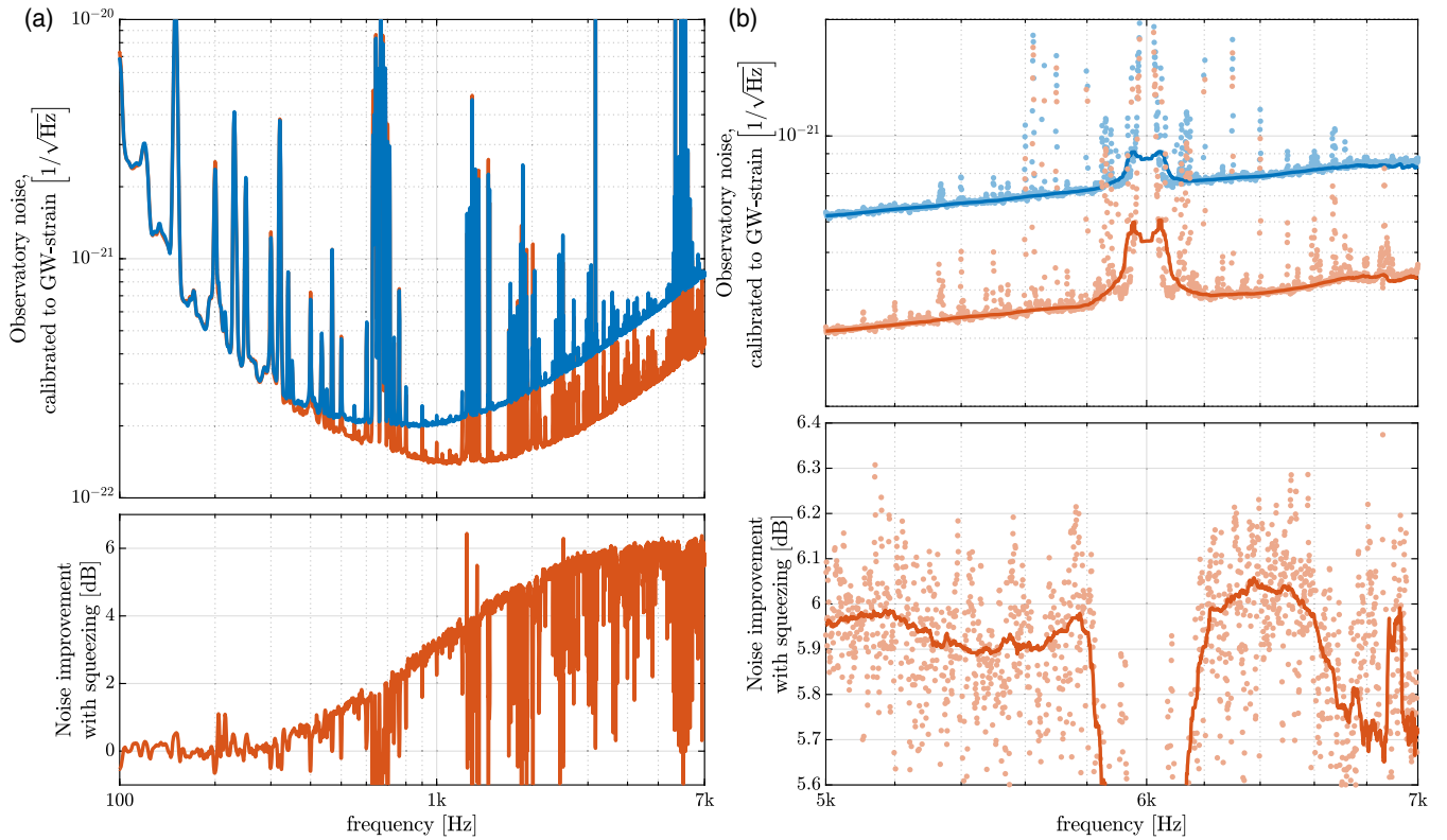
FIG. 2. With the application of squeezing, we observe a factor of 2 improvement in sensitivity at high frequencies. (a) The top plot compares 15 minute power spectral density (PSD) estimates of the detector noise with (red) and without (blue) squeezing. Towards higher frequencies, the increase in shot noise proportional to f is due to calibration compensation of the filtering effect of the SRC. The bottom plot shows the squeezing ratio as a function of frequency. The squeezing value of 6.03 \pm 0.02 dB is calculated from the ratio between median noise floor estimates with and without squeezing averaged between 6.3 and 6.5 kHz and referenced against periods where the squeezing was not applied during valid science time over a two month duration. Toward lower frequencies, the squeezing is increasingly limited by technical noise. Plot (b) shows a zoomed-in section of the same data (dots). Noise floor estimates in the top plot and their ratio in the bottom plot are depicted as solid lines.
