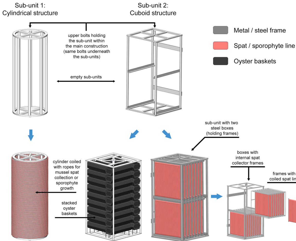
Fig. 5. Sub-units of the Shellfish Tower . On the left (cylindrical) spat collecting / sporophyte coil devices are shown while on the right (cuboid) sub-units can either host oyster baskets piled up on top of each other or units for holding frames with coiled spat lines.
