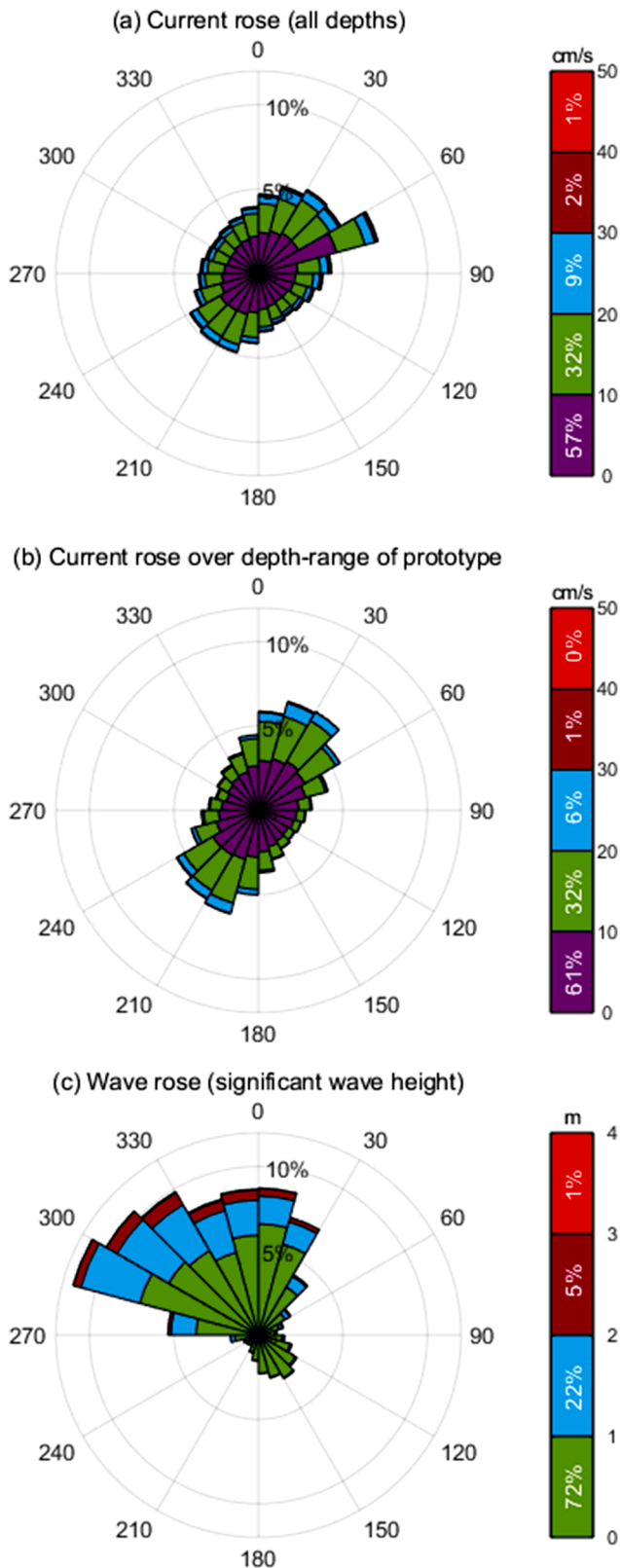
Fig. 3. (A) Current conditions (velocity in cm/s), throughout water column (B) current conditions (velocity in cm/s) over deployment depth of prototype and (C) Significant wave height ( H_s in m) and wave direction at test site. Note that directionality of currents is in the ‘going to’ sense while wave direction is given in the ‘coming from’ sense.
