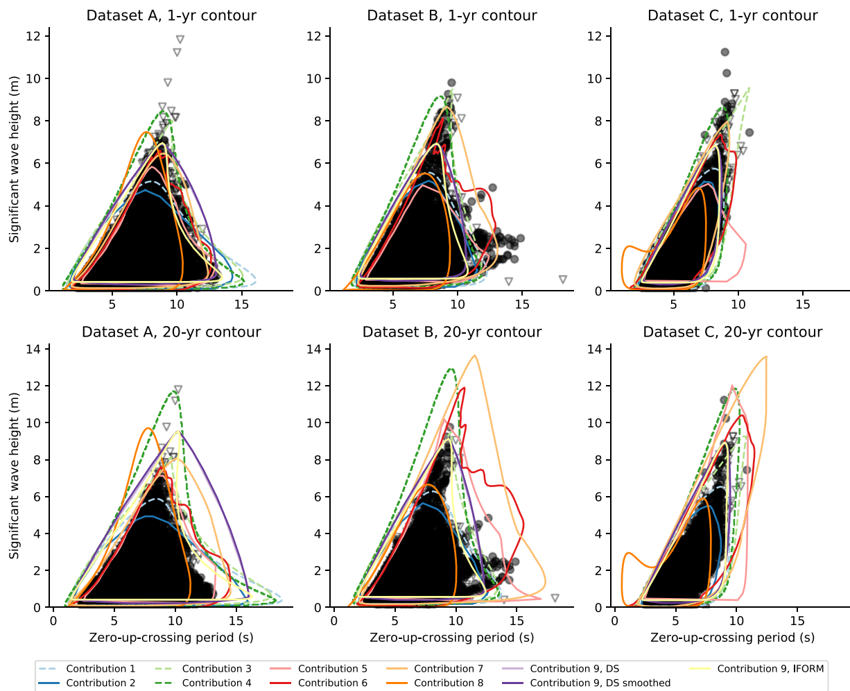
Fig. 11. Exercise 1, datasets A, B, C: contour overlays. — = marginal exceedance contours, - - = total exceedance contours, ◦ = provided data (10 years), ▽ = retained data (10 years).
