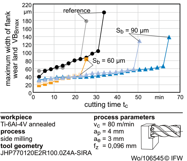
Fig. 15 Results of the wear tests on Ti-6Al-4V
