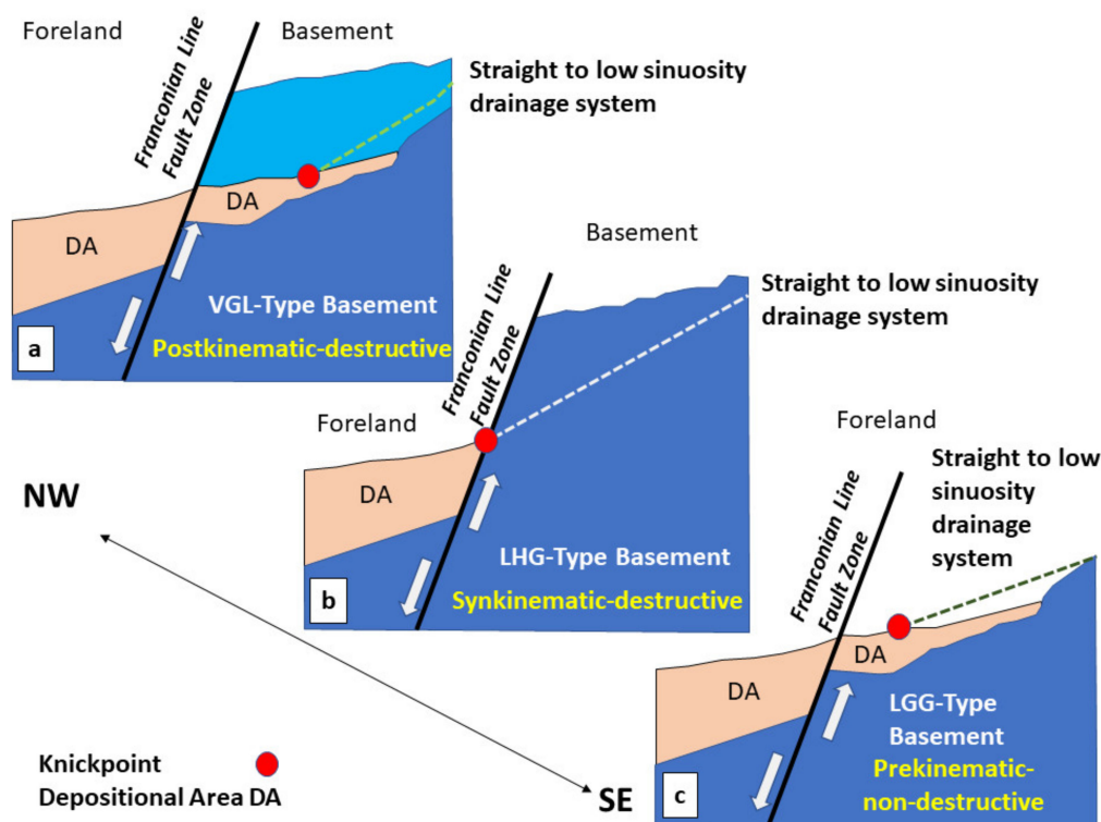
Figure 17. Cartoon to illustrate the relation between Cenozoic fault kinematic along the Franconian Line Fault Zone (FLFZ) and the evolution of the straight to low sinuosity drainage systems of the basement in the various reference sites from NW to SE. The 1st order knickpoint is indicated by the red dot. (a) VGL-Type; (b) LHG-Type; (c) LGG-Type.
