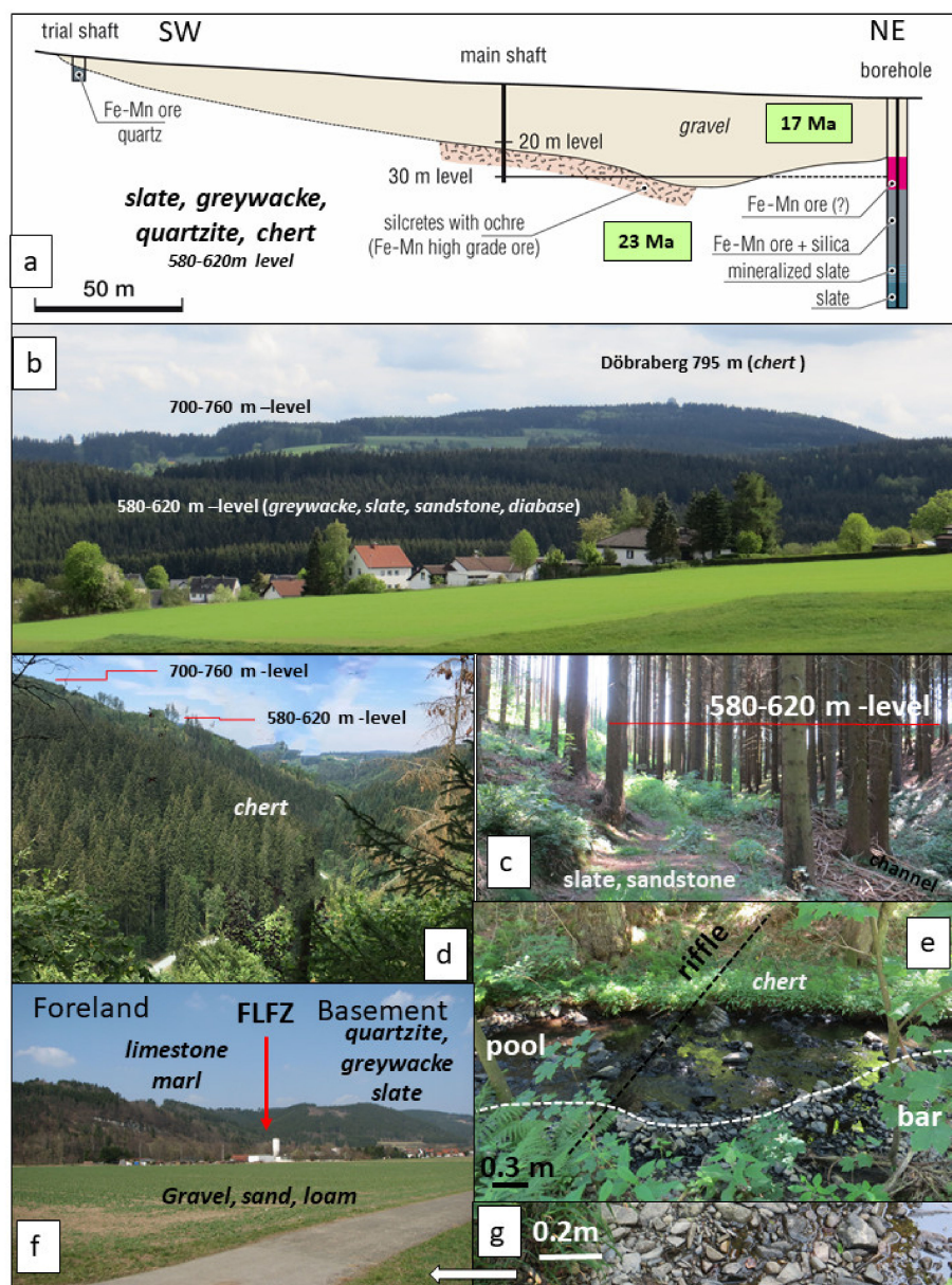
Figure 6. Fluvial landforms from the CA, TA and DA of the VLG-type (Table 1). For penneplains, erosional and depositional terraces, and floodplains see Figure 3. (a) Wide-and-shallow valley of the proto-drainage system (penneplain in the CA) filled with coarse-grained alluvial-fluvial deposits and Fe-Mn ore. The age of formation of the cryptomelane at the bedrock-valley floor and as cement are given in green boxes. (b) The monadnock of the Döbraberg representative of a relic penneplain in the CA. A wide-and-shallow valley in the foreground (see also (a)). (c) Wide-angle single-channel alluvial V-shaped valley evolved in loamy regolith near the watershed (slope angle 15^\circ \Rightarrow 20^\circ , talweg angle 3.3^\circ \Rightarrow 1.2^\circ ). (d) Incision of the acute-angle single-channel non-alluvial V-shaped valley of the Wilde Rodach into the Neogene penneplains (slope angle 30^\circ \Rightarrow 35^\circ , talweg angle 2.7^\circ \Rightarrow 0.7^\circ ) (photograph by courtesy of H. Schmalfuss). (e) Close-up view of the channel of (d) with steps and pools in Devonian chert (stippled white line = strike of bedding) and the onset of wandering channels to evolve. (f) Transition from the TA into the DA while crossing the Franconian Lineamentary Fault Zone (FLFZ) between the uplifted basement and the foreland at the 440–500 m level (modern floodplain = 340 m). A U-shaped valley with steep slopes and wide flood plain evolved between paired terraces (slope angle/ basement 30^\circ \Rightarrow 35^\circ , talweg angle 0.3^\circ \Rightarrow 0.2^\circ ), in places > 35^\circ ; slope angle/ foreland 25^\circ \Rightarrow 30^\circ , talweg angle 0.2^\circ \Rightarrow 0.3^\circ ). (g) Close-up view of the flood plain deposits (mainly greywacke, quartzite) of (f).
