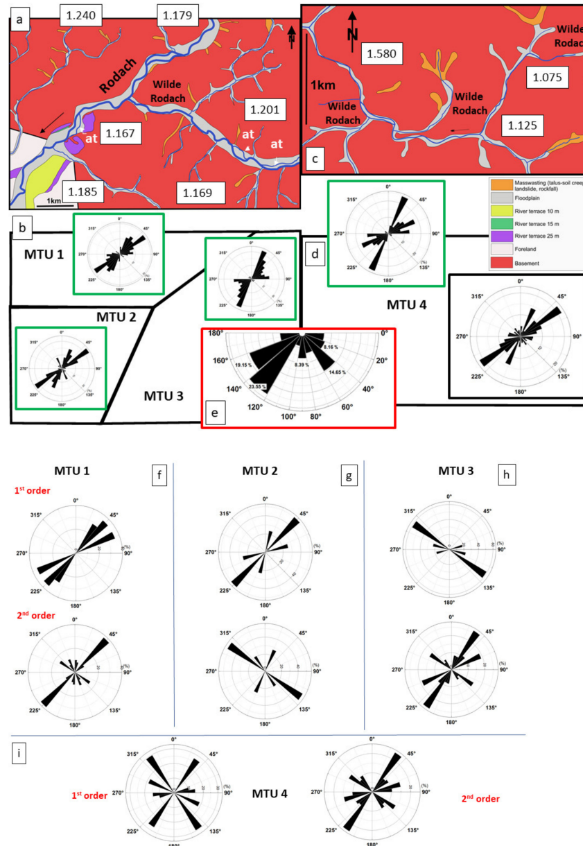
Figure 8. Litho- and morphotectonic units (MTU) characterized by the sinuosity of drainage systems (rectangular boxes) and the structural geology of the bedrock in VLG-type (see Figure 3). Fold structures (a–e) in full-circle rose diagram framed in green shows the cleavage and full-circle rose diagram framed in black shows the main fault zones (520 data). (a) DA and TA of the VLG-type drainage systems; (b) Tectonic datasets for (a) (MTU 1, MTU 2 and MTU 3); (c) TA and CA of the VLG-type drainage systems; (d) Tectonic dataset for (c) (MTU 4); (e) Composite semicircle rose diagram showing the orientation and frequency of faults in the Frankenwald within the Teuschnitz Syncline and the Berga Anticline (Figure 1b); (f) Orientation of 1st and 2nd order fluvial channels of MTU 1 (percentage of total length of the drainage system); (g) Orientation of 1st and 2nd order fluvial channels of MTU 2 (percentage of total length of the drainage system); (h) Orientation of 1st and 2nd order fluvial channels of MTU 3 (percentage of total length of the drainage system); (i) Orientation of 1st and 2nd order fluvial channels of MTU 4 (percentage of total length of the drainage system).
