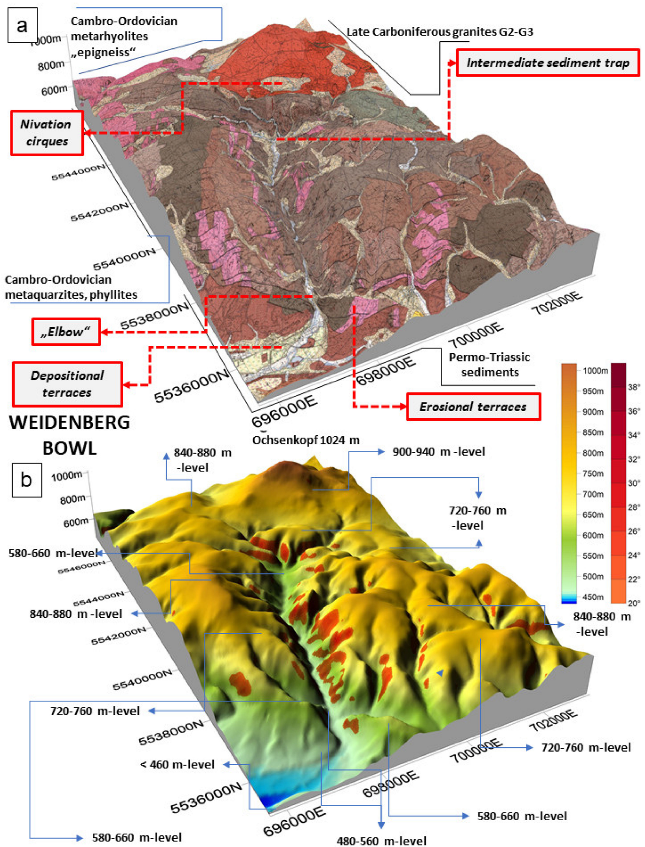
Figure 5. The drainage system of the Fichtelgebirge Anticline (Table 1-LGG-type): (a) Geology and the geomorphological setting; (b) Excerpt of the topography and the level of paleosurfaces of (a).
