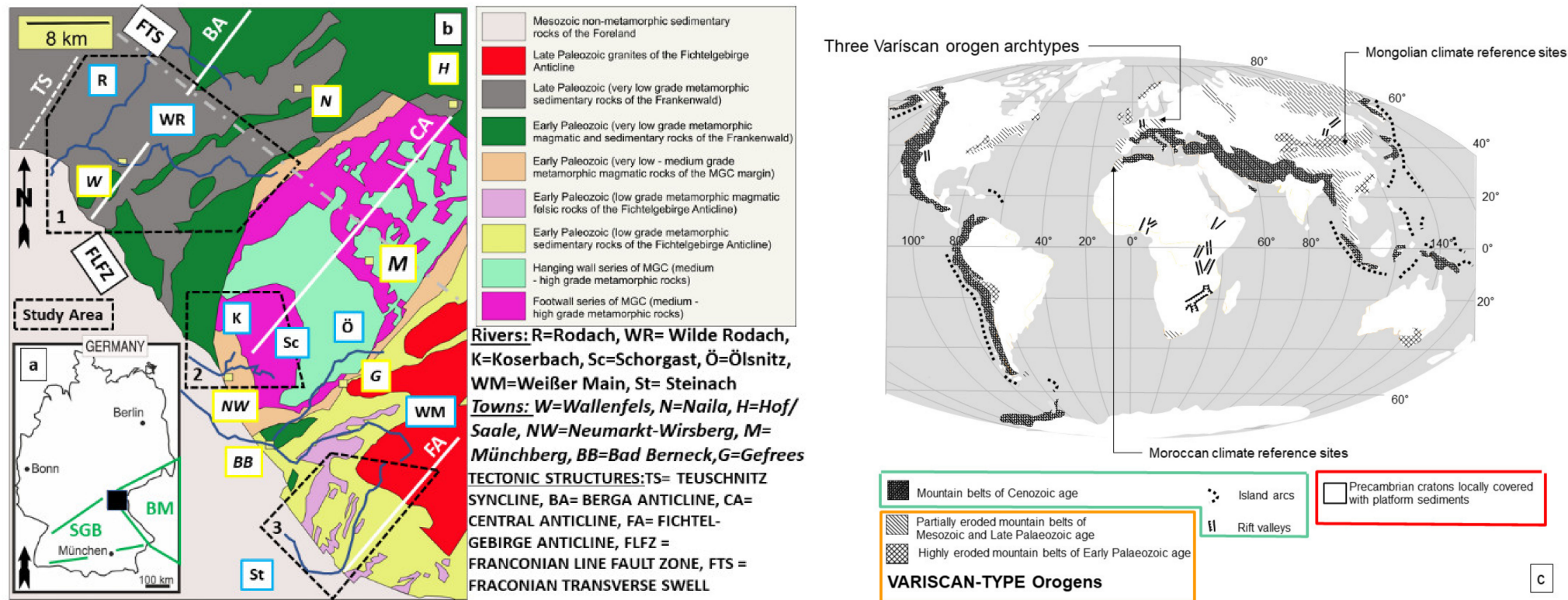
Figure 1. Position and the geological setting of the study area in SE Germany with three type localities framed by stippled line: 1. VLG-type area, 2. LHG-type area, 3. LGG-type area. For features of each reference site see Table 1. (a) Position of the study area in the Central European Variscides in SE Germany at the NW edge of the uplifted basement of the Bohemian Massif (BM) and at the NE margin of the South German Block (SGB) representative of the Mesozoic and Cenozoic foreland basin. Rivers, towns and tectonic structures as well as geology are shown on the right-hand side, (b) The geological setting of the three type localities at the NW edge of the Bohemian Massif. Geological basis [35] (c) The position of the study areas referred to in the text in relation to the geomorphological-geodynamic setting and the distribution of Variscan-type orogens Maturity of crustal section: green: pre-mature, orange: mature, red: super-mature [36].
