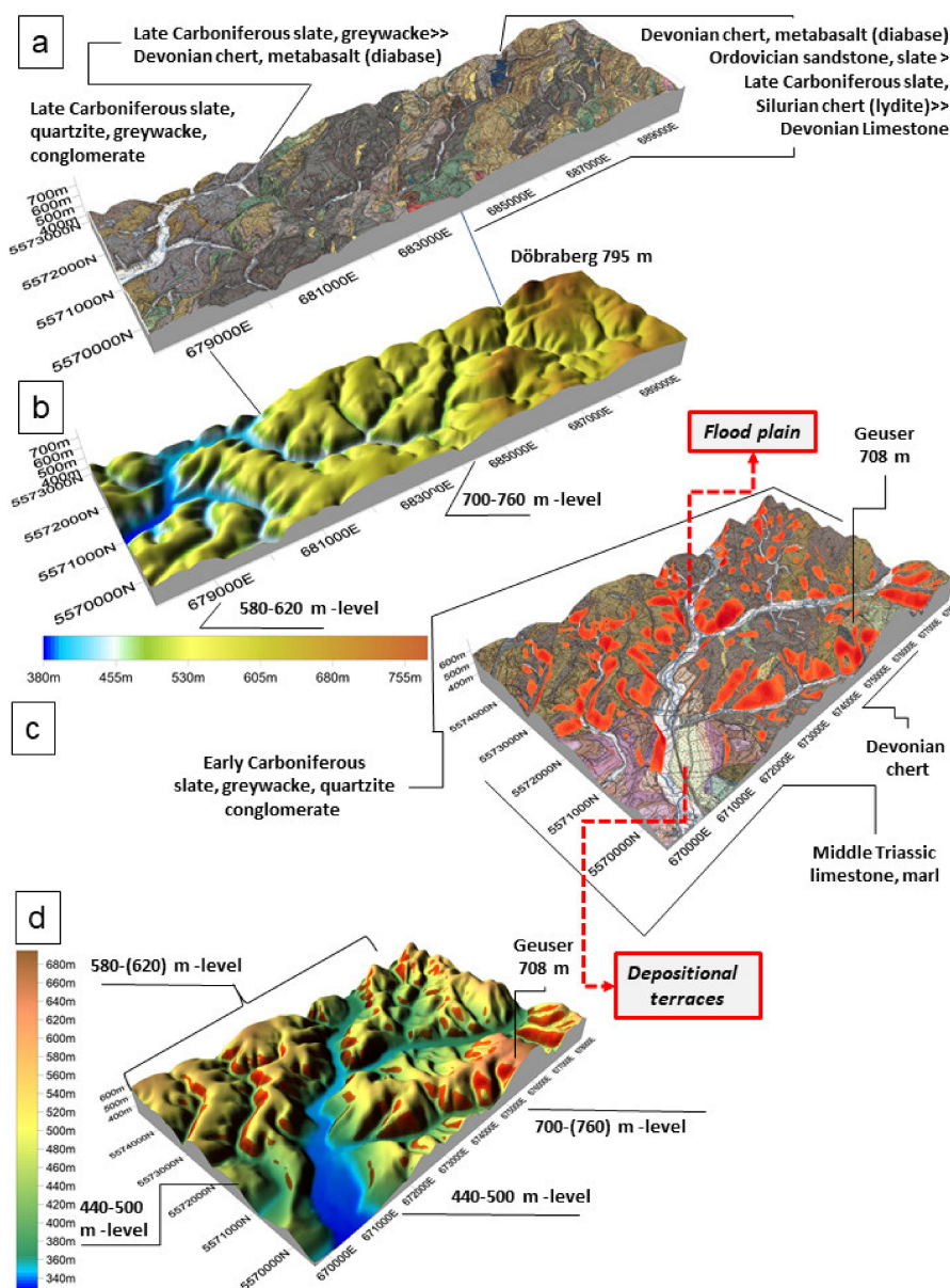
Figure 3. The drainage system in the Frankenwald (FW) (Table 1-VLG-type) in digital terrain models (DTM) The V-shaped valleys are highlighted by the slope angle shaded in red (see angle bar = midslope). Rectangles framed in red denote landforms of fluvial relevance. (a) Geology and the geomorphological setting in the upper reaches (headwaters = (CA)) transitional into the proximal transport area (TA)); (b) Excerpt of the topography and the level of paleosurfaces of (a); (c) Geology and the geomorphological setting in the lower reaches (distal TA transitional into the depositional area (DA) within the basement and proximal foreland); (d) Excerpt of the topography and the level of paleosurfaces of (c).
