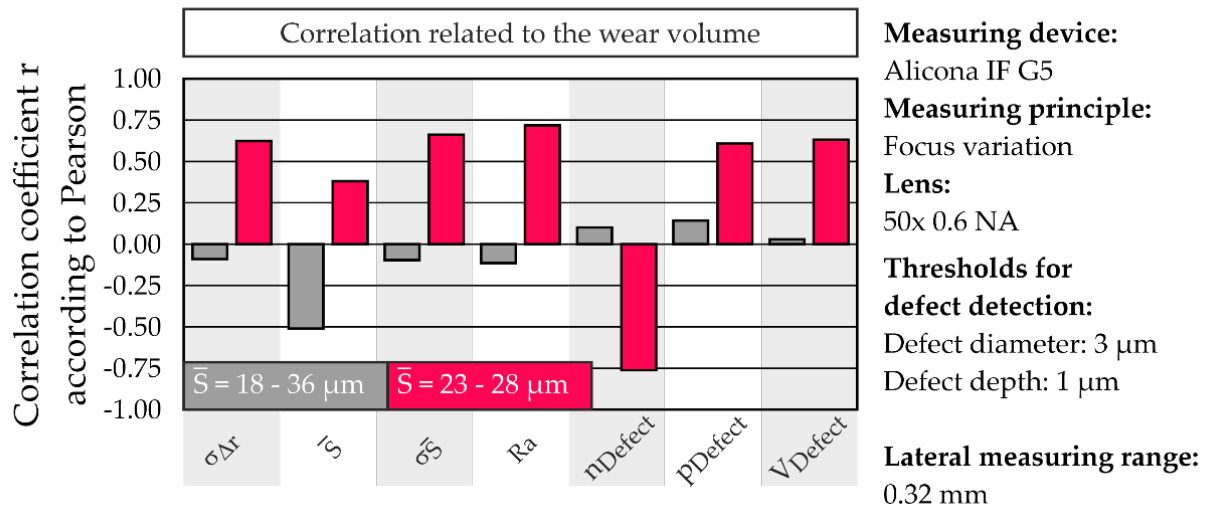
Figure 12 gives an overview of the calculated Pearson coefficients between the different edge quality characteristics and the mean wear volume, depending on the considered parameter range of the cutting edge rounding.
