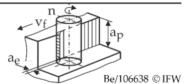
Figure 12. Correlation between the chipping parameters and the wear volume.
