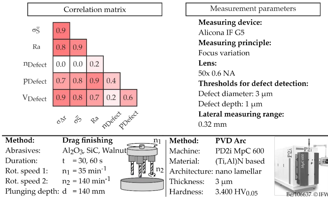
Figure 10. Correlation of different parameters for the description of the chipping.
