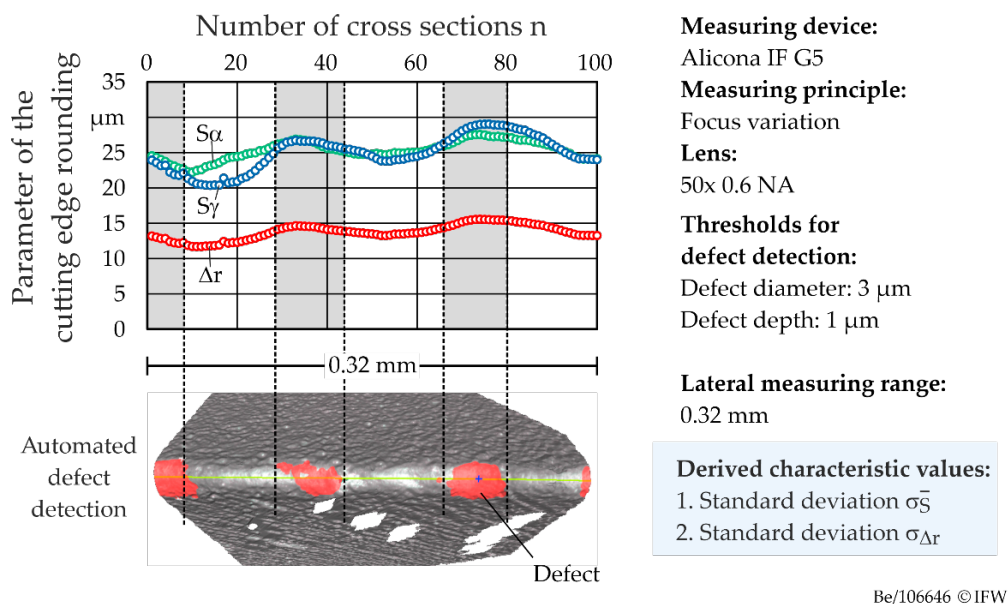
Figure 11. Correlation between the parameters characterizing cutting edge rounding and the defective areas along the cutting edge.
