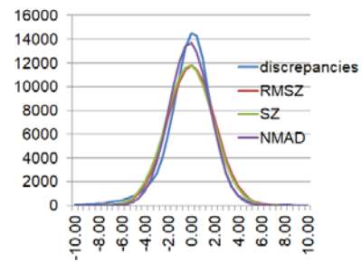
Figure 12. Frequency distribution of AW3D30 discrepancies improved by ZFIT and filtered against LiDAR
