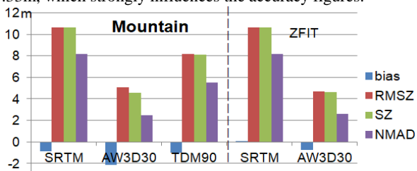
Figure 14. Accuracy results in test site Mountain
