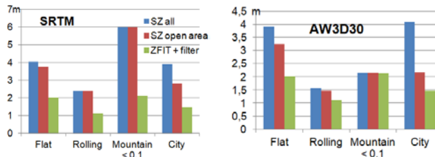
Figure 24. Standard deviation of SRTM and AW3D30 DSM
