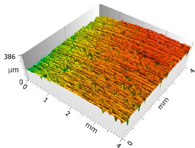
Fig. 10 3D scan of the sharpened grinding layer
