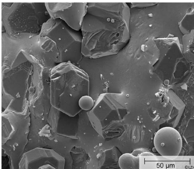
Fig. 7 SEM image (side view) from parameter set 1
