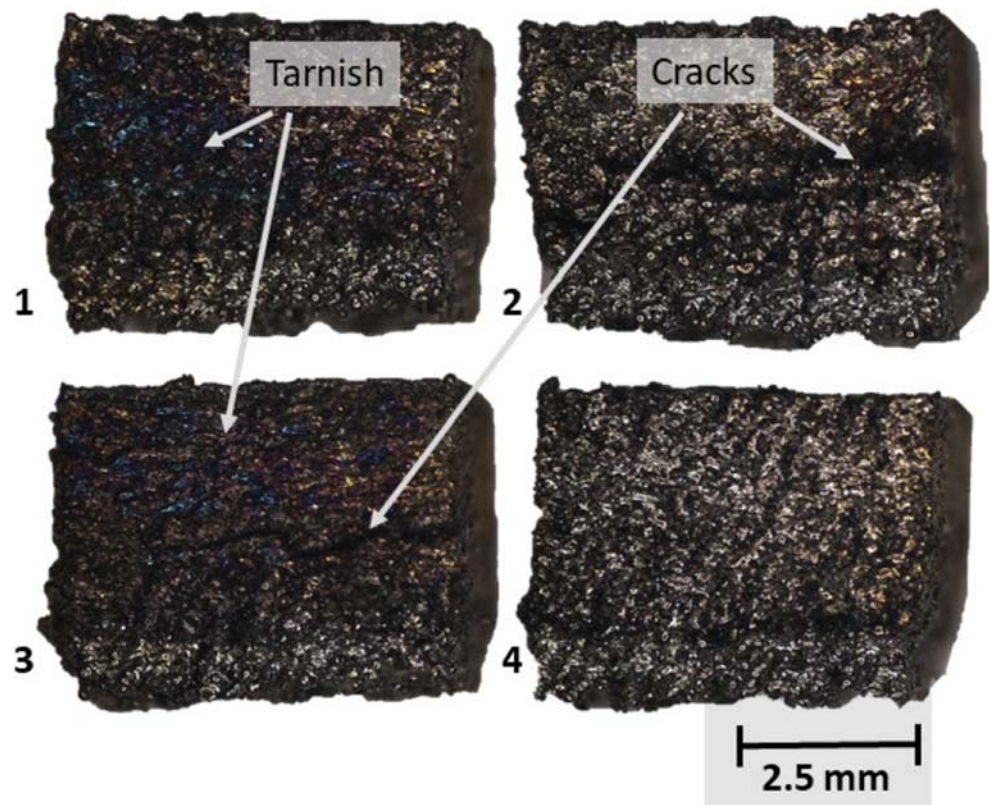
Fig. 6 Photography of LPBF manufactured test samples with dispersed diamonds. Numeration as in Table 2
