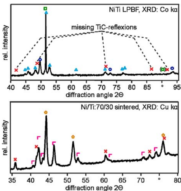
XRD Target: Co, Cu samples I LPBF NiTi II sintered Ni/Ti:70/30 T_s = 1100\text{ }^\circ\text{C} t_s = 300\text{ s} symbols × TiC □ CDia ○ NiTi cub. ▢ TiNi 3 ▲ NiTi mart. ● Ni Km/94723 ©IFW
