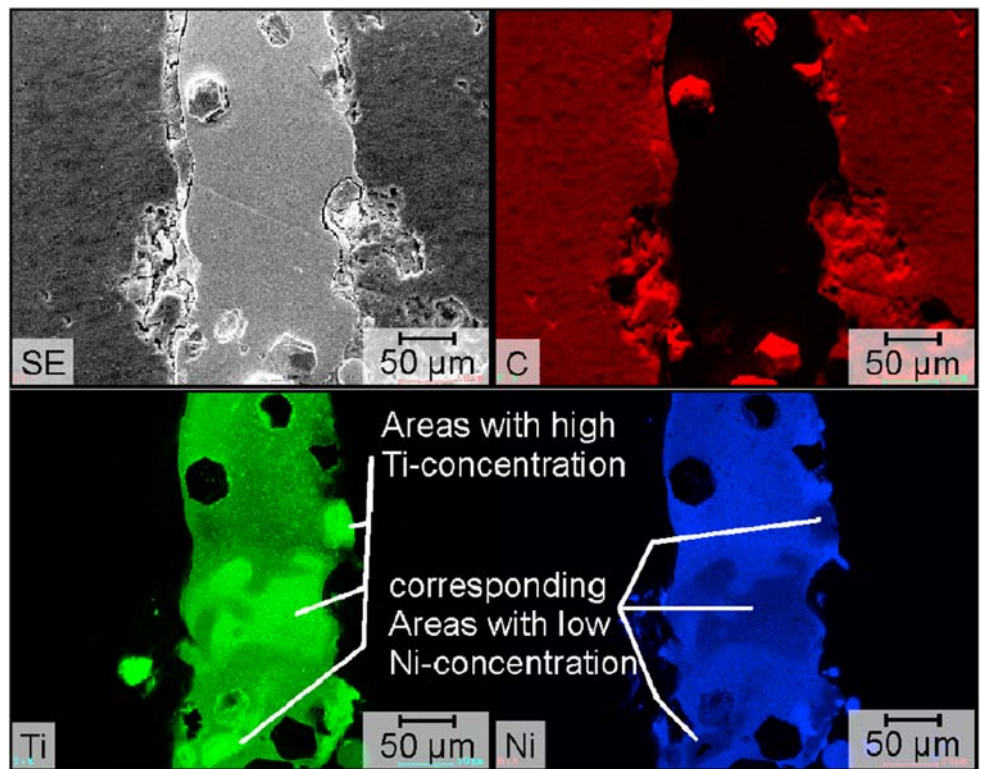
Fig. 4 Distribution of elements in the line can trials of powder #1
