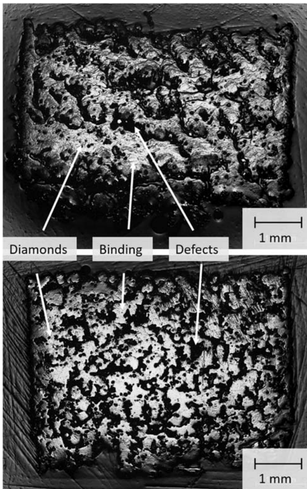
Fig. 8 Light microscope images of cross sections of samples built with the parameter sets 1 (top) and 4 (bottom)
