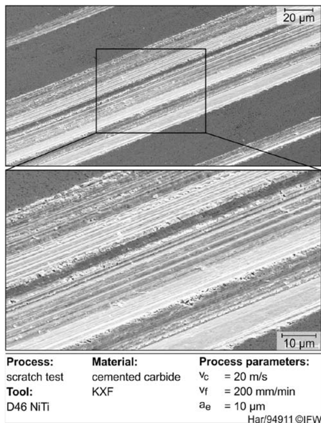
Fig. 11 SEM picture of scratch paths
