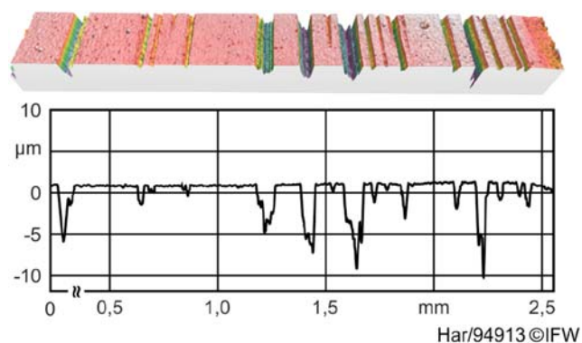
Fig. 12 Laser scan of scratch paths
