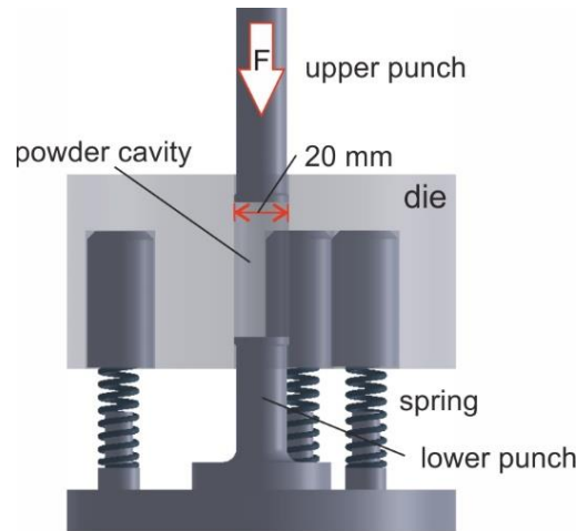
Figure 1 Experimental setup
