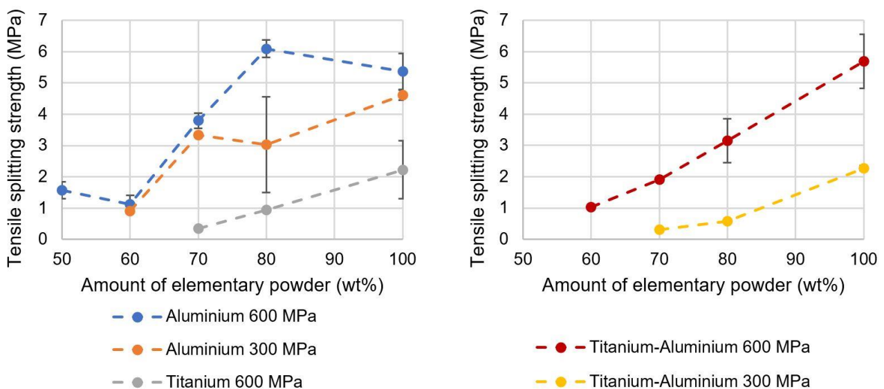
Figure 3 Tensile splitting strength as a function of different proportions of elemental titanium or aluminum powder (left), titanium and aluminum powder (right)
