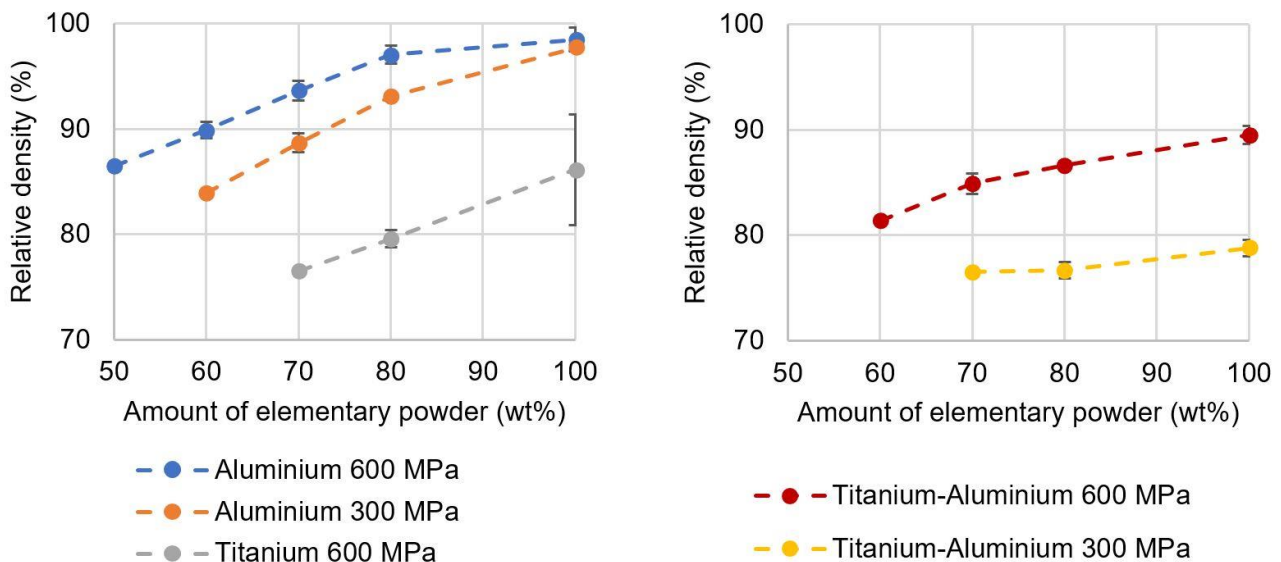
Figure 2 Relative density as a function of different proportions of elemental titanium or aluminum powder (left), titanium and aluminum powder (right)
