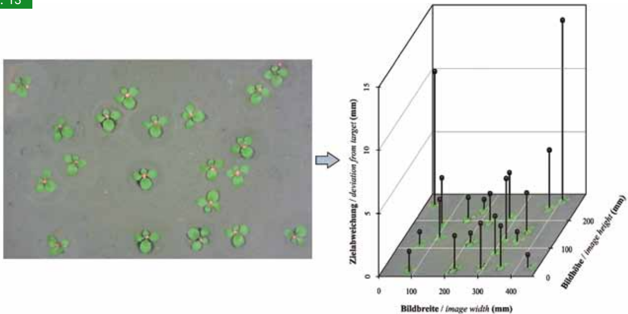
Test of the system with 20 positioned weed plants (image processing and positioning of the laser beam) (Photos: T. Rath)
