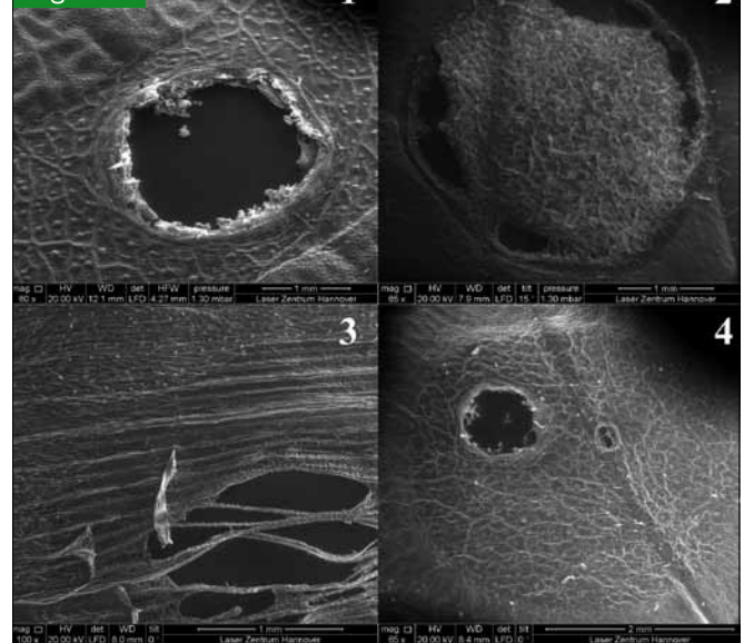
REM images of laser-irradiated leaves (Photos: Ch. Marx) 1: Diamond K-500, CO 2 -laser (λ = 10 600 nm), energy: 8.9 J, spot diameter: ø 3 mm 2: 48-5 (Synrad Inc.), CO 2 -laser (λ = 10 600 μm), energy: 7.1 J, entire spot diameter: ø 3 mm with ø 200 μm focused beam 3: SpitLight DPSS 250 (InnoLas GmbH), solid-state laser (λ = 532 nm), energy: 1 ns pulse with 125 mJ, spot diameter: ø 6 mm 4: LDF 600-250 (Laserline GmbH), diode laser (λ = 940 nm), energy: 70.8 J, spot diameter: ø 6 mm
