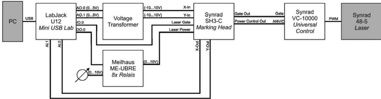
Schematic diagram for control of galvanometer-servo motors (Drawing: Ch. Marx)
