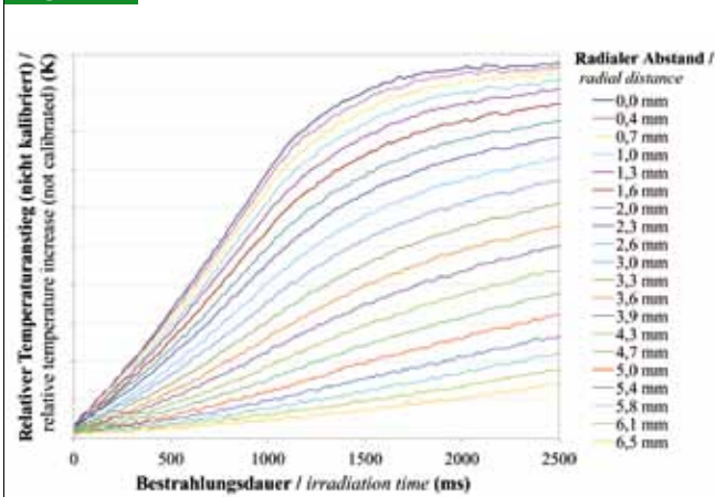
Presentation of thermal measurements with radial distance to the aim spot center during constant irradiation (CO 2 -laser, λ = 10 600 nm, 3.5 W)
