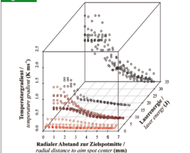
Influence of applied laser energy (Gauß-beam with ø 6 mm) on temperature gradient relative to the aim spot center
