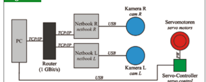
Linking of the system components
