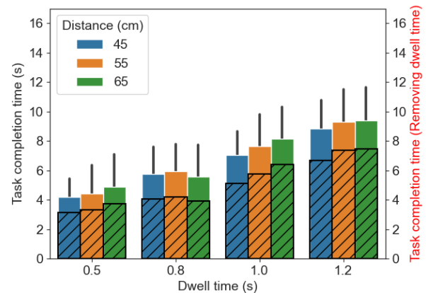
Figure 8. The average task completion time. The error bars represent the standard deviation in each condition. The striped bars are the task completion time after removing the duration of the dwell time.
