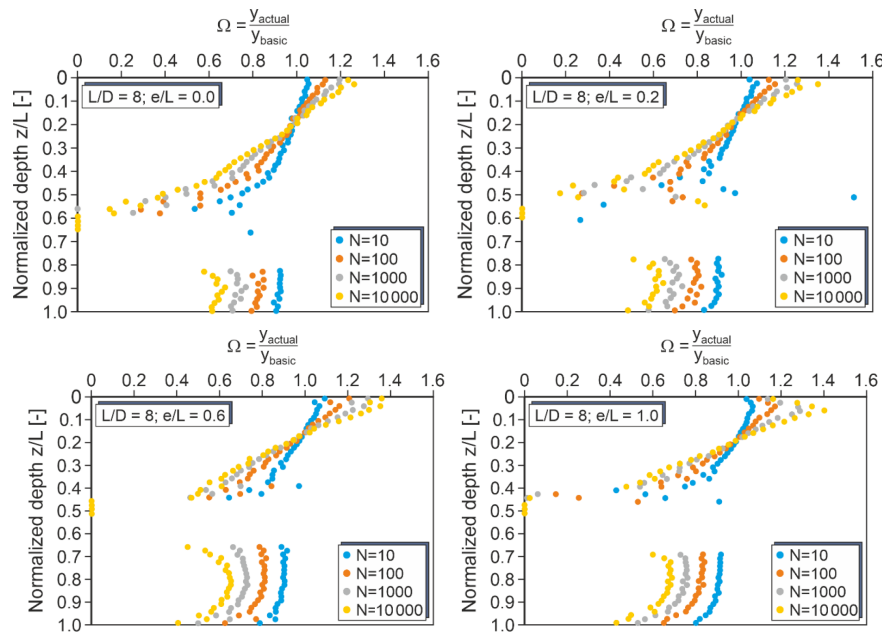
Figure 13. Correction factors \Omega for monopiles with L/D = 8 and different load eccentricities (very dense sand).
