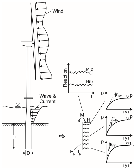
Figure 1. Monopile foundation of an offshore wind energy converter and p - y method used in design (schematic).
