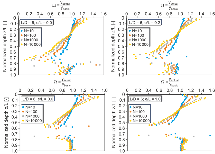
Figure 11. Correction factors \Omega for monopiles with L/D = 6 and different load eccentricities (very dense sand).
