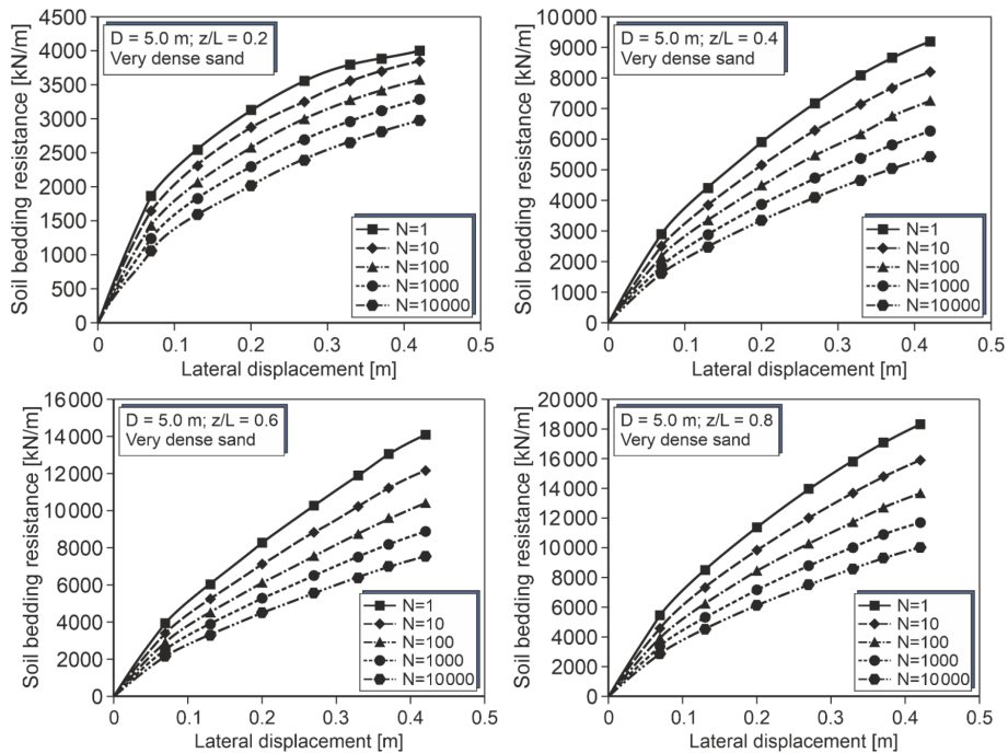
Figure 5. p - y curves for different cycle numbers (monopile D = 5 m, L = 25 m, very dense sand).
