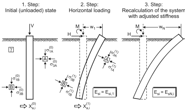
Figure 3. Calculation steps of the stiffness degradation method.
