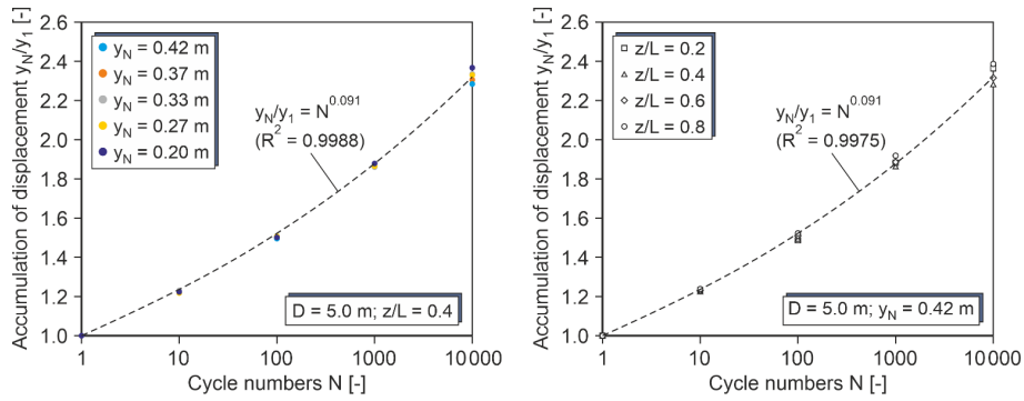
Figure 6. y multipliers for a monopile D = 5 m, L = 25 m in very dense sand.
