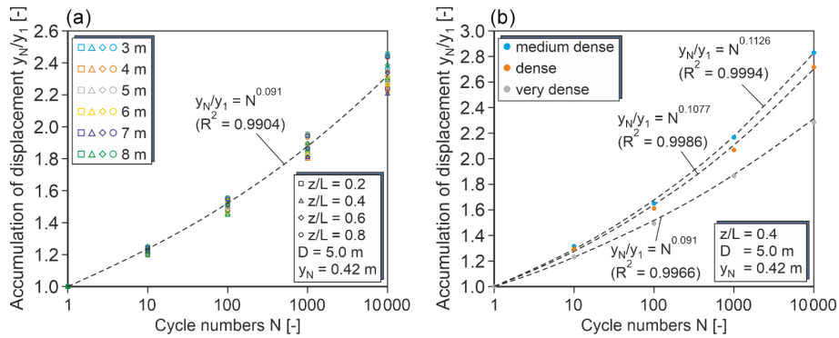
Figure 7. y multipliers for variable pile diameters (a) and for different relative densities of the sand (b).
