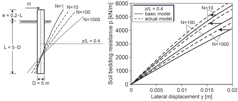
Figure 9. Exemplary comparison of p - y curves for constant horizontal displacement (bold lines) and p - y curves for the actual configuration (monopile in very dense sand).
