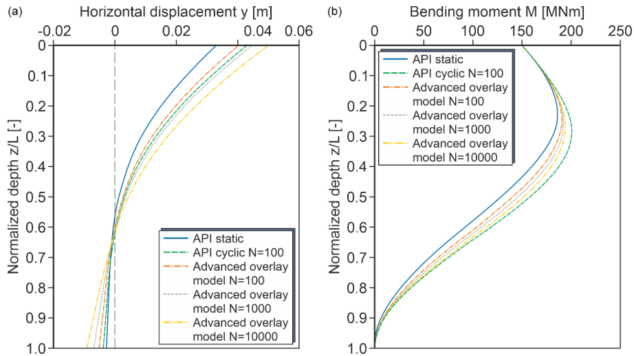
Figure 14. Comparison of pile deflection lines (a) and bending moments (b).
