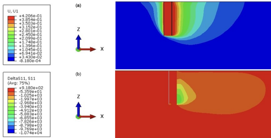
Figure 4. Horizontal displacements (a) and stresses (b) for a monopile D = 5 m under static load in very dense sand ( N = 1 , prescribed pile displacement y = 0.42 m).
