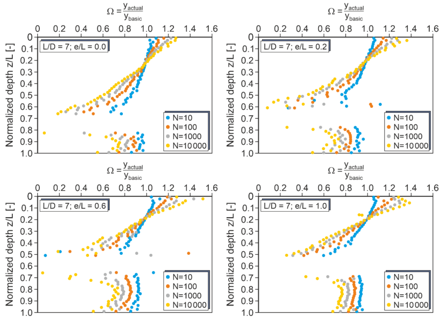
Figure 12. Correction factors \Omega for monopiles with L/D = 7 and different load eccentricities (very dense sand).
