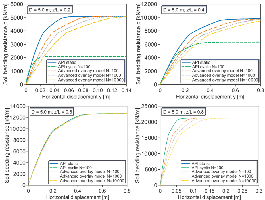
Figure 15. Comparison of cyclic p - y curves
