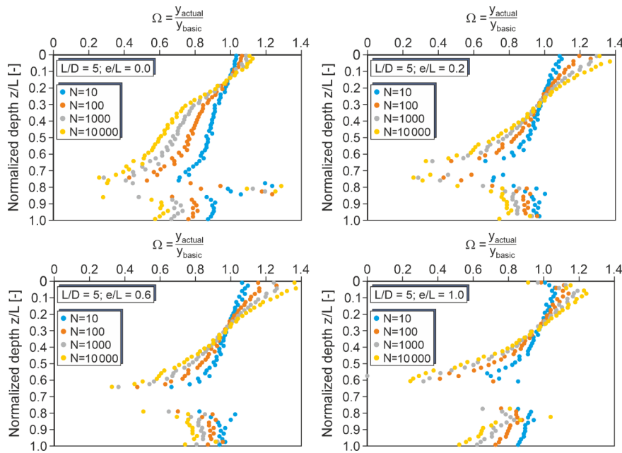
Figure 10. Correction factors \Omega for monopiles with L/D = 5 and different load eccentricities (very dense sand).
