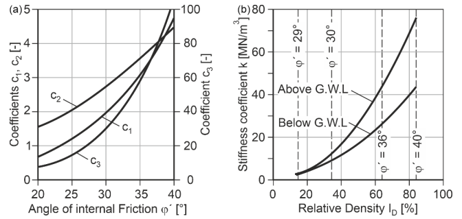
Figure 2. Coefficients C_1 , C_2 and C_3 (a) and parameter k (b) according to API (2014).
