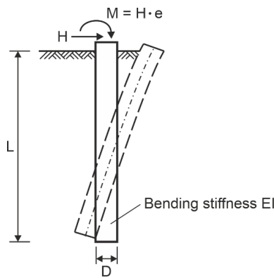
Figure 8. System and applied loading for the advanced overlay model.
