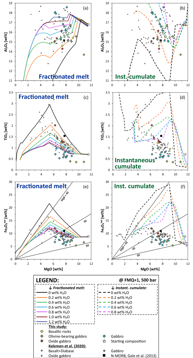
Figure 14. \text{Al}_2\text{O}_3 , \text{TiO}_2 and \text{Fe}_2\text{O}_3^{\text{tot}} versus \text{MgO} for bulk major element compositions of drill hole GT3A lithologies (data from this study and from Kelemen et al., 2020). (a, c, e) Solid lines represent fractional crystallization modeling using MELTS for varying initial \text{H}_2\text{O} contents. (b, d, f) Dashed lines represent the instantaneous cumulate corresponding to the sum of the crystallized phases formed within a temperature interval of 20^\circ\text{C} for different initial \text{H}_2\text{O} contents. Starting composition is listed in Table 2. For details see text.
