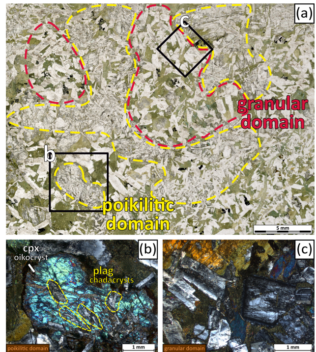
Figure 4. (a) Thin-section photo of varitextured gabbro GT3A-55Z-4, 38–43 cm; plane-polarized light. Poikilitic and granular domains are highlighted. The marked boxes represent details shown in (b) and (c). (b) Poikilitic texture: lath-shaped plagioclase (plag) chadacrysts are enclosed by clinopyroxene (cpx) oikocrysts; cross-polarized light. (c) Granular texture: assemblages of tabular plagioclase and hornblende; cross-polarized light.
