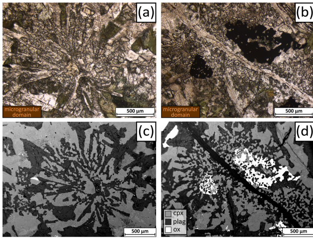
Figure 7. Rosette-like, microgranular domains within two varitextured gabbros ( a, c : GT3A-129Z-3, 50–57 cm; b, d : GT3A-129Z-4, 8–16 cm) consisting of radiating granular clinopyroxenes and lath-shaped plagioclases, sometimes associated with interstitial Fe–Ti oxides ( b, d ). For details see text. ( a, b ) Microphotographs in plane-polarized light; ( c, d ) backscattered electron images.
