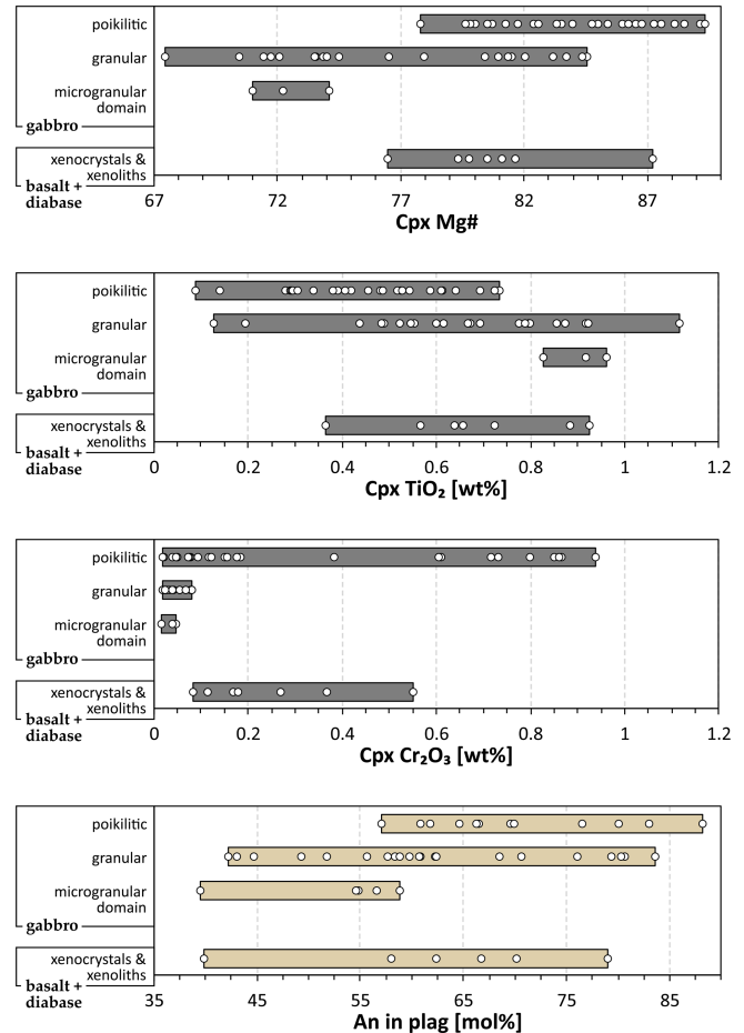
Figure 8. Range of compositions (bars) and averages (white circles) of clinopyroxene and plagioclase recorded in different textural domains. Compositional variation in Mg#, TiO 2 and Cr 2 O 3 in clinopyroxene, showing higher values in the poikilitic domains except for TiO 2 , which is consistent with the more primitive nature of the poikilitic domains. Clinopyroxenes from microgranular domains show significantly lower Mg#’s. Since the compositional zoning is significantly narrower in clinopyroxenes compared to plagioclase, bars include core measurements. The compositional variation in An contents from core measurements shows higher values in the poikilitic domains overlapping with the granular domains.
