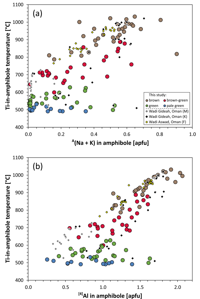
Figure 11. Relationship between tetrahedral Al and Na + K on the A position of the amphiboles versus the Ti-in-amphibole temperature for the different groups, classified by mineral color. Also shown are amphibole data as comparison from other locations of the most southern blocks of the Oman ophiolite: Wadi Gideah (M: Müller et al., 2017, frozen AML; K: Koepke et al., 2022, layered gabbro) and Wadi Aswad (F: France et al., 2021). The amphiboles from the crustal level of a frozen AML show both low tetrahedral Al and ^A(\text{Na} + \text{K}) together with a lower Ti-in-amphibole temperature. In contrast, the layered gabbros from Wadi Gideah exhibit much more scattering, whereas the amphibole data from Wadi Aswad exhibit higher Ti-in-amphibole temperature for tetrahedral Al and ^A(\text{Na} + \text{K}) , showing an overlap with the brown and brown-green amphiboles from this study.
