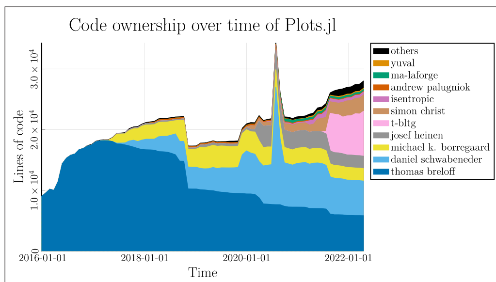
Figure 6 Lines of code alive of the top ten contributors of the Plots.jl repository over time. Data created with hercules [36].
