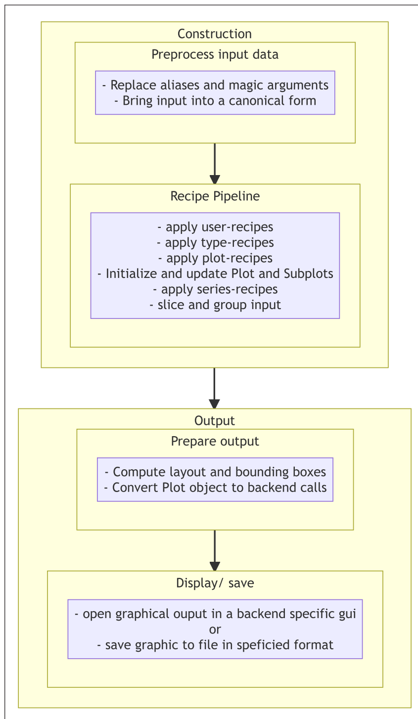
Figure 2 Plotting pipeline in Plots.jl . The separation of construction and output production enables the flexible use of different backends in the same session and helps to avoid unnecessary intermediate calculation. Created using mermaid [1].
