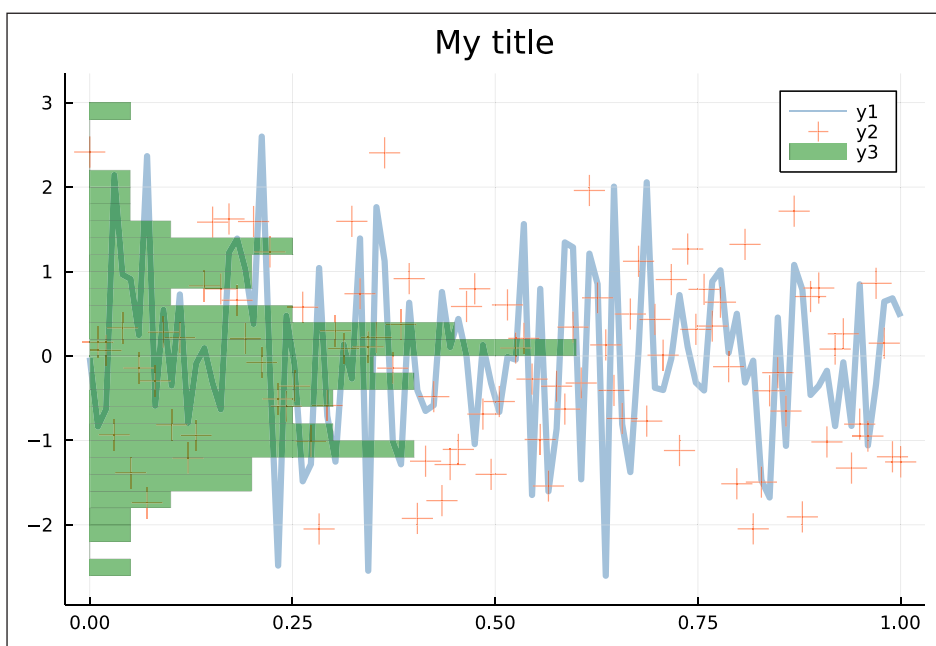
Figure 5 An example figure generated from the code shown in Listing 6. Listings 7 and 8 illustrate how the generated backend code could look like for different backends. The actual backend code is more verbose and likely uses more low-level functions. These listings also show how Plots.jl provides a unified API for its backend packages, since the translation between Listings 7 and 8 is not straightforward.
