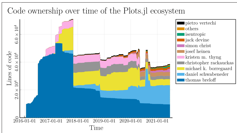
Figure 7 Lines of code alive of the top ten contributors of the Plots.jl ecosystem (Figure 4) over time. Data created with hercules [36].
