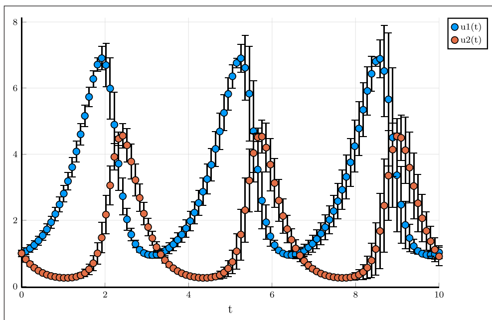
Figure 3 Showcase of composing recipes. Plotting a ODESolution object from DifferentialEquations.jl containing Measurements from Measurements.jl will apply the recipe of DifferentialEquations.jl which will return vectors of Measurements , which will apply the recipe from Measurements.jl ; yielding the solutions of the Lotka-Volterra system [2] with correct error bounds without the user having to change the callsite. Neither of these packages has code in their recipes for handling types of the other package. Full code available in Listing 9 .
