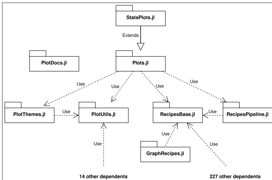
Figure 4 Overview of the Plots.jl ecosystem and its interfaces with other Julia packages. The numbers of dependents are taken from juliahub [30].
