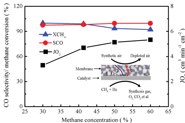
Fig. 8 Influence of methane concentration on CH 4 conversion (▲), CO selectivity (●) and oxygen permeation flux (■) through the 40NSFO–60CNO dual phase membrane without an LSC coating on the air side in the POM to synthesis gas. Conditions: feed side: fair = 150 cm 3 min -1 , sweep side: F He + F CH 4 + F Ne = 20 cm 3 min -1 , 1 cm 3 min -1 Ne as internal standard gas, membrane thickness: 0.6 mm. Temperature: 950 °C.
