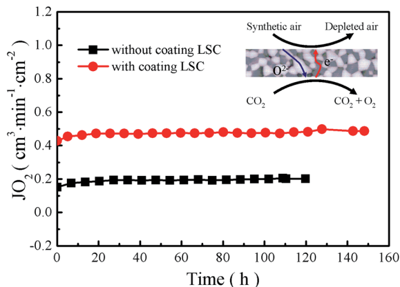
Fig. 6 Oxygen permeation flux through the 40NSFO–60CNO dual phase membrane as a function of time with pure CO 2 as the sweep gas for membranes without and with porous LSC coating. Conditions: 150 cm 3 min -1 air as feed gas, 49 cm 3 min -1 CO 2 as sweep gas; 1 cm 3 min -1 Ne as internal standard gas. Membrane thickness: 0.6 mm. Temperature: 950 °C.
