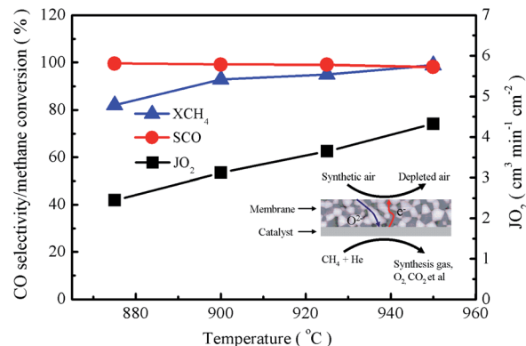
Fig. 7 Influence of temperature on CH 4 conversion (▲), CO selectivity (●) and oxygen permeation flux (■) through the 40NSFO–60CNO dual phase membrane without LSC coating on the air side in the POM to synthesis gas. Conditions: 150 cm 3 min -1 air as feed gas, 11 cm 3 min -1 He with 8.27 cm 3 min -1 CH 4 as sweep gas; 1 cm 3 min -1 Ne as internal standard gas. Membrane thickness: 0.6 mm.
