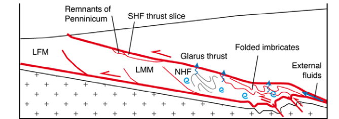
Fig. 9. (Colour online) Schematic cross-section illustrating the (a) diagenetic to (b) metamorphic evolution of the Infracalcare flysch units during the Alpine orogeny. LFM – Lower Freshwater Molasse; LMM – Lower Marine Molasse; NHF – North-Helvetic flysch; SHF – South-Helvetic flysch; UHF – Ultrahelvetic flysch. The blue arrows indicate fluid flow; the blue spirals indicate internal fluid evolution. Based on Burkhard et al. (1992), Dielforder et al. (2016) and Pfiffner (1986). Not to scale.
