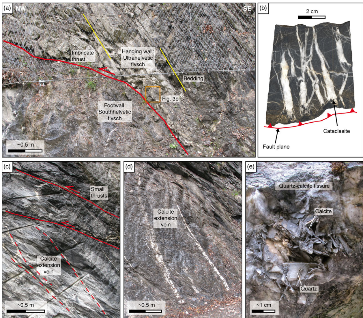
Fig. 3. (Colour online) (a) Tectonic contact between Ultrahelvetetic flysch (hanging wall) and South-Helvetetic flysch (footwall). (b) Example of calcite extension veins formed in the direct hanging wall of the imbricate thrust fault shown in (a). The veins contain fragments of a cataclasite that formed along the imbricate thrust. (c) Example of small thrusts cross-cutting calcite extension veins in the footwall of the imbricate thrust. (d) Example of steep calcite extension veins in the footwall. (e) Mineralized fissure with euhedral quartz and calcite crystals. Sampling site: 46.9597° N, 9.1881° E.
