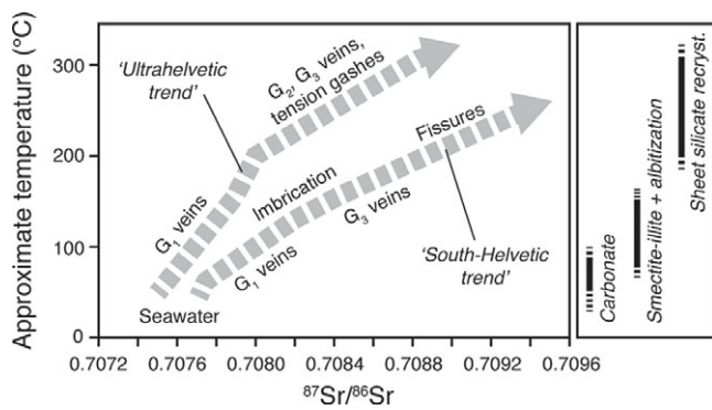
Fig. 8. (Colour online) Diagram illustrating the Sr isotopic evolution of pore fluids in the Ultrahelvetic flysch and South-Helvetic flysch units. The increase from the seawater-like signature towards more radiogenic values is interpreted to relate to diagenetic and metamorphic processes, including carbonate diagenesis, smectite-to-illite transformation, alkali-feldspar albittization, illite-to-muscovite transformation and recrystallization (recryst.) of detrital white mica and biotite. See Sections 5.a and 6 for details.
