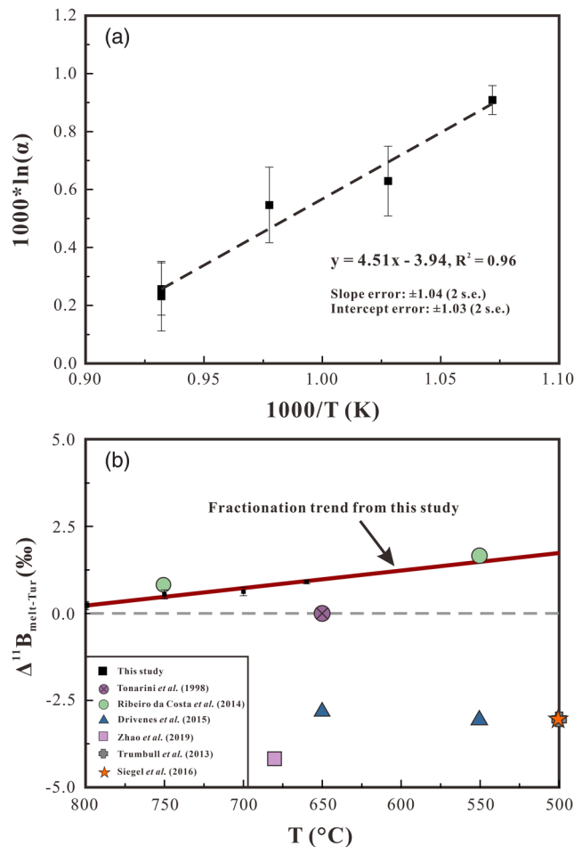
Figure 2 (a) Boron isotopic fractionation factors between granitic melt and tourmaline versus reciprocal temperature. The dashed line represents an Ordinary Least Square regression of the five fractionation values obtained from our experiments. (b) Comparison of \Delta^{11}\text{B}_{\text{melt-Tur}} values from this study and \Delta^{11}\text{B}_{\text{melt-Tur}} applied in previous studies to interpret \delta^{11}\text{B} values analysed in tourmaline.
