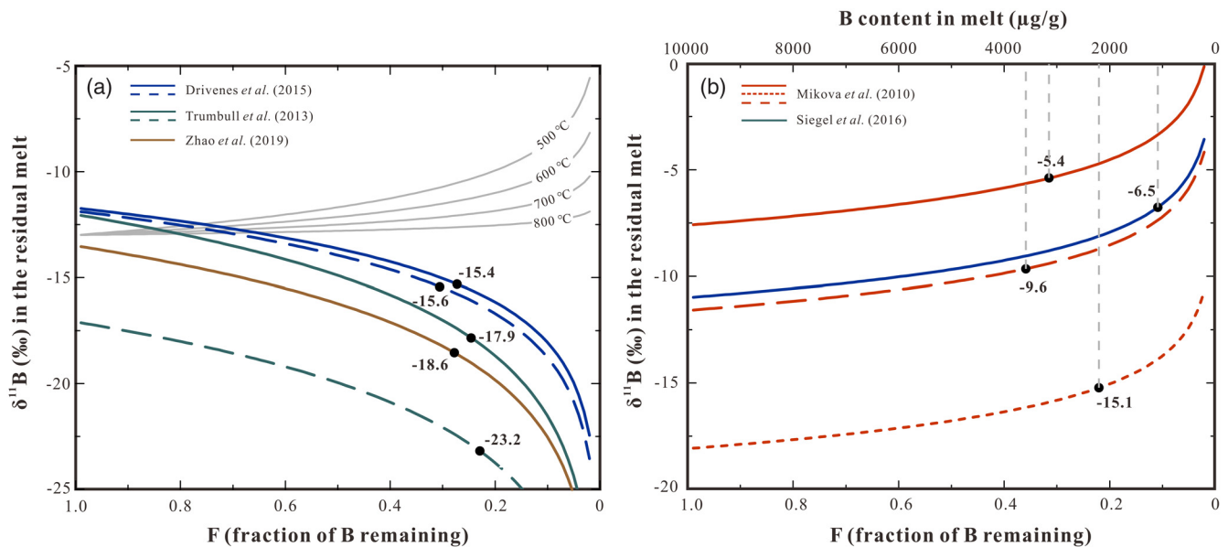
Figure 3 (a) Modelled curves illustrating the change in \delta^{11}\text{B} values for residual melt after crystallisation of tourmaline, assuming a Rayleigh fractionation. Grey solid curves represent the evolution in \delta^{11}\text{B} assuming tourmaline crystallisation, the starting \delta^{11}\text{B} values of the melt are set as -13\text{‰} and the fractionation factors are based on the result of this study. The coloured lines are calculated \delta^{11}\text{B} variation trends of residual melts based on the \delta^{11}\text{B} analyses of zoned tourmalines and negative \Delta^{11}\text{B}_{\text{melt-Tur}} fractionation factors applied in the studies of Trumbull et al. (2013), Drivenes et al. (2015), and Zhao et al. (2019) (see data in Table S-8). Note the discrepancy between the grey solid lines and the coloured lines. (b) Rayleigh fractionation model illustrating the variation of \delta^{11}\text{B} of residual melt with ongoing tourmaline crystallisation using tourmaline data from Mikova et al. (2010) and Siegel et al. (2016) and the positive fractionation factors from this study. The black dots in both figures represent \delta^{11}\text{B} values of melt at the end of tourmaline crystallisation, calculated from the \delta^{11}\text{B} values determined at the rim of the tourmalines. The \delta^{11}\text{B} values at F = 1.0 are calculated from \delta^{11}\text{B} values determined in the core of the tourmalines. Data used to draw the coloured lines are listed in Table S-8, and the detailed calculation process is given in SI.
