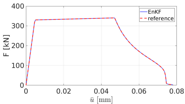
Fig. 15 The load-displacement curve for the ductile fracture problem in Example 5, estimated by the inferred values
