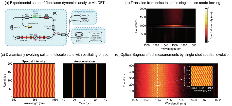
Figure 7. Examples of fiber laser evolution dynamics characterized via DFT analysis over hundreds of cavity roundtrips. (a) Experimental setup for the study of a fiber laser exhibiting soliton-soliton dynamics via DFT. (b) Single pulse mode-locking obtained after a transition from a noisy operation and an explosion regime (white dashed box), with an abrupt spectral broadening clearly captured by DFT measurements. (c) DFT measurements can be used to study the dynamical evolution of a soliton molecular state. The spectra evolution can be used to retrieve autocorrelations of the field, stemming from a ‘molecule state’ with a periodically oscillating phase. Panels (a-c) are adapted from [91]. (d) Experimental observation of the Sagnac effect in a bidirectional fiber laser, illustrated by a change in the tilted modulation pattern within the DFT spectra. Adapted from [103].
