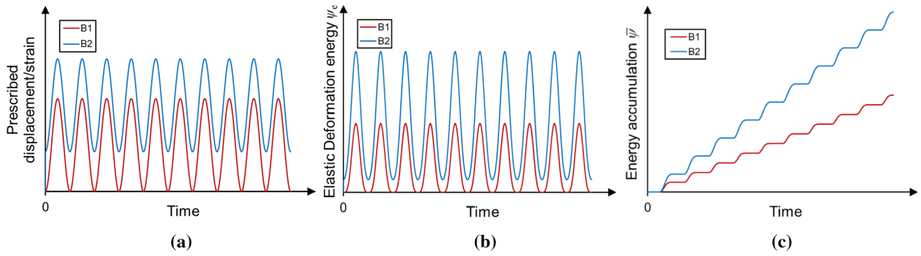
Fig. 6 a Prescribed load, b resulting elastic deformation energy and c energy accumulation variable of 1D bar subjected to sinusoidal displacement-controlled loading with different mean values
