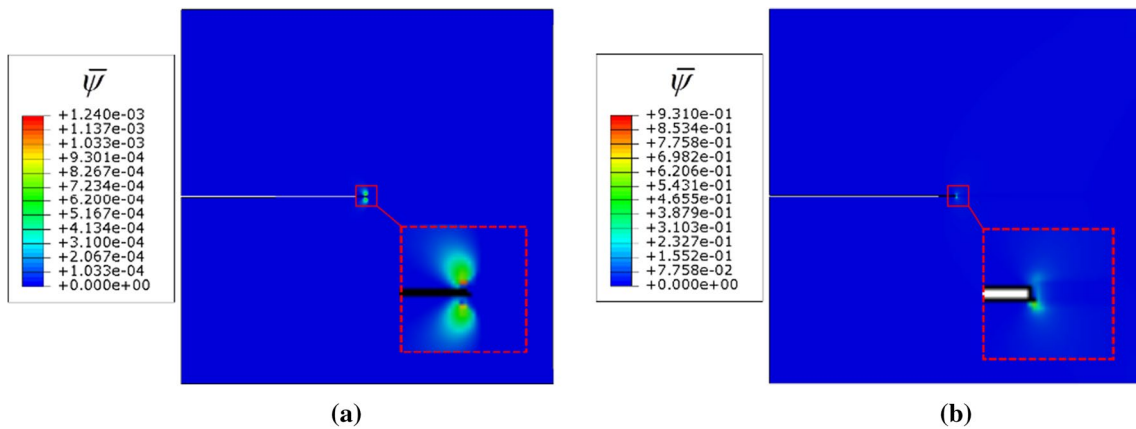
Fig. 14 Energy accumulation variable in MPa a before and b after the formation of crack
