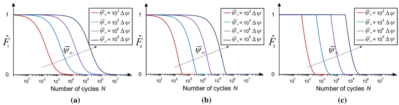
Fig. 7 Influence of parameter \bar{\psi}_\infty for three different fatigue degradation functions a \hat{F}_1 , b \hat{F}_2 , c \hat{F}_3
