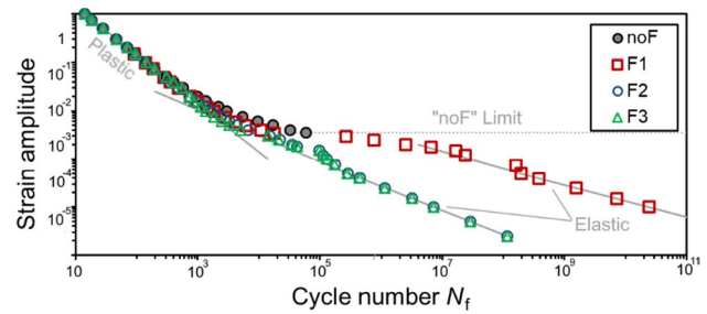
Fig. 17 Cyclically loaded round bar specimen. \epsilon - N curve
