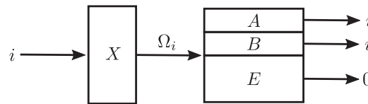
Figure 6. Example of a protocol for a secret sharing scheme: a sender X chooses a state \Omega_i from the set of code states \{\Omega_0 = \Omega, \Omega_X, \Omega_Z, \Omega_Y\} and sends it to the system consisting of authorised shares Alice ( A ) and Bob ( B ) and unauthorised share Eve ( E ). The shares then operate locally on their part of the system to detect which state they received. The authorised shares Alice and Bob will be able to recover the information i of which state they received, whereas Eve will always get the same answer (0) no matter which state was sent.
