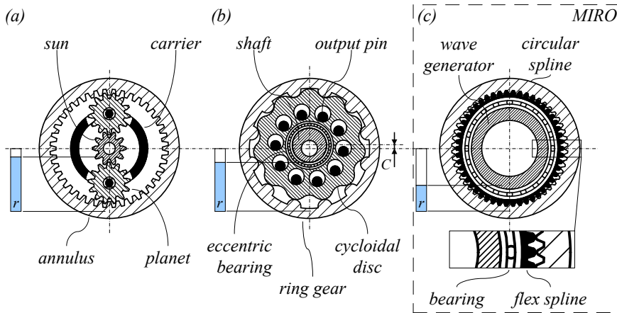
Figure 4.35: Three reduction gear principles: planetary speed reducer (a), cycloidal speed reducer (b), Harmonic Drive reduction gear (c)
