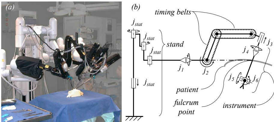
Figure 3.9: The da Vinci ® Surgical System ( Intuitive Surgical ® Inc.): Three arm robotic setup (a), kinematic chain of a single telemanipulator (b)
