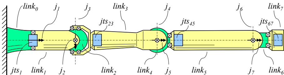
Figure 4.39: Overview of the joint torque sensor integration in the MIRO (bearings of j_2 , j_4 , and j_6 not depicted)
