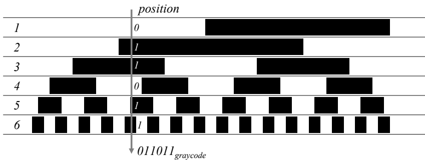
Figure C.8: 6 bit graycode
