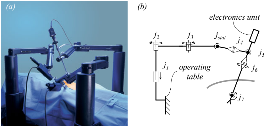
Figure 3.10: The Zeus ® telerobotic system: Three arm configuration at the operation table, picture courtesy of Intuitive Surgical ® Inc. (a), kinematic chain of a single telemanipulator (b)
