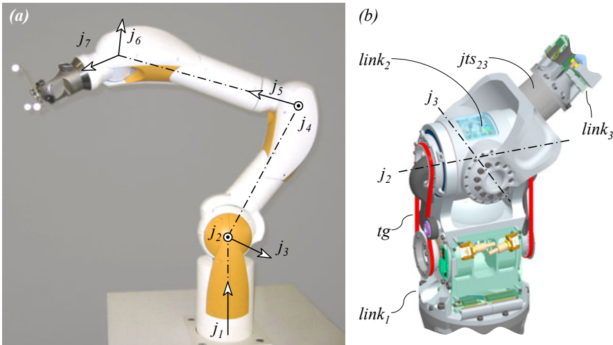
Figure D.2: The KineMedic robot equipped with a marker array for intraoperative navigation systems, picture courtesy of BrainLAB AG (a), rendering of the 2-DoF couple joint for j_2, j_3 based on bevel gears (b)
