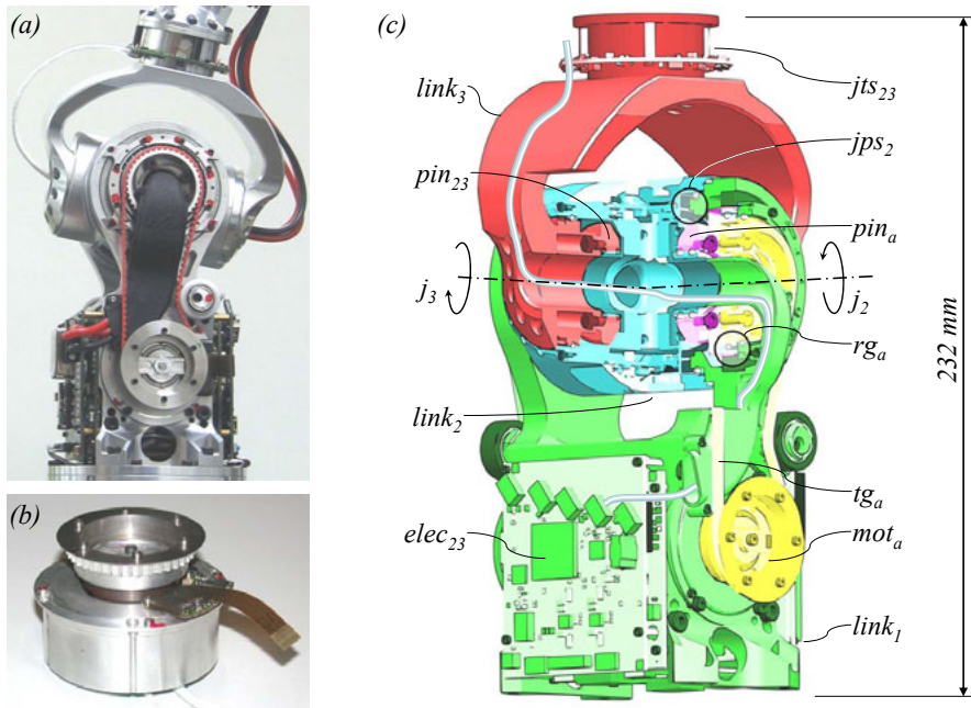
Figure 4.57: The miro 23 joint module (a), motor module ( mot ), integrating motor, motor position sensor, brake, and timing belt gear (b), rendered view (differential gear portion as cross-section) with stationary parts ( link 1 ) highlighted in green, parts coupled with link 2 in blue, joint-sided parts ( link 3 ) in red, high-speed motor parts are shown in yellow (c)
