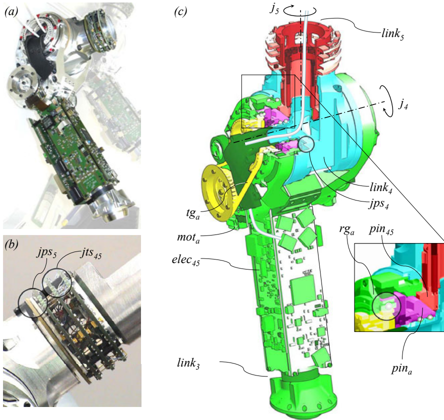
Figure 4.58: The miro 45 joint module (a), module integrating the joint-sided torque and position sensors ( jts 45 , jps 5 ) (b), rendered view (differential gear portion as cross-section) with stationary parts ( link 3 ) highlighted in green, parts coupled with link 4 in blue, joint-sided parts ( link 5 ) in red, high-speed motor parts in yellow (c)
