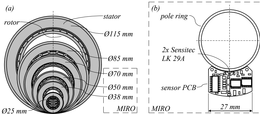
Figure 4.44: Diameter range of the ILM motor (a), the MR-sensor for commutation (b)
