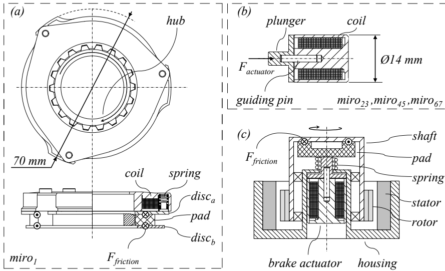
Figure 4.47: Brakes of the MIRO robot: MAYR RSM-70 for miro_1 (a), brake actuator for miro_{23} , miro_{45} , miro_{67} (b), simplified depiction of the brake actuator integration in miro_{23} and miro_{45} (c) (note: drawings (a), (b), and (c) have different scaling)
