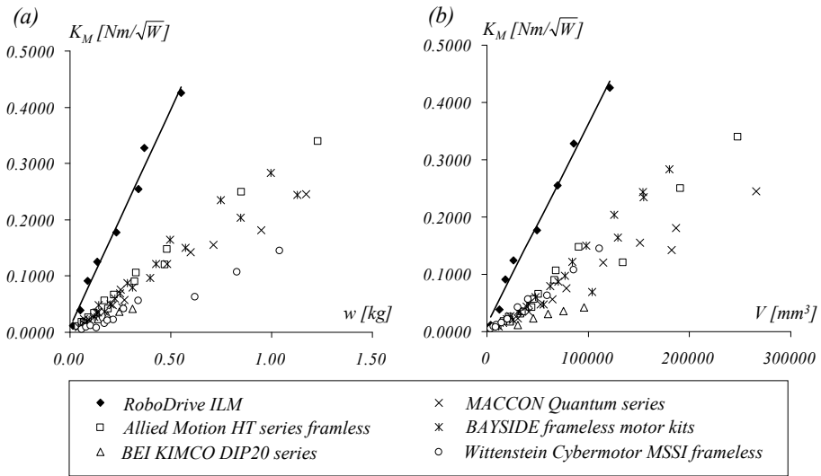
Figure 4.45: Comparison of various BLDC motors: motor constant K_M with respect to weight w [kg] (a), motor constant K_M with respect to volume V [mm 3 ] (b)
