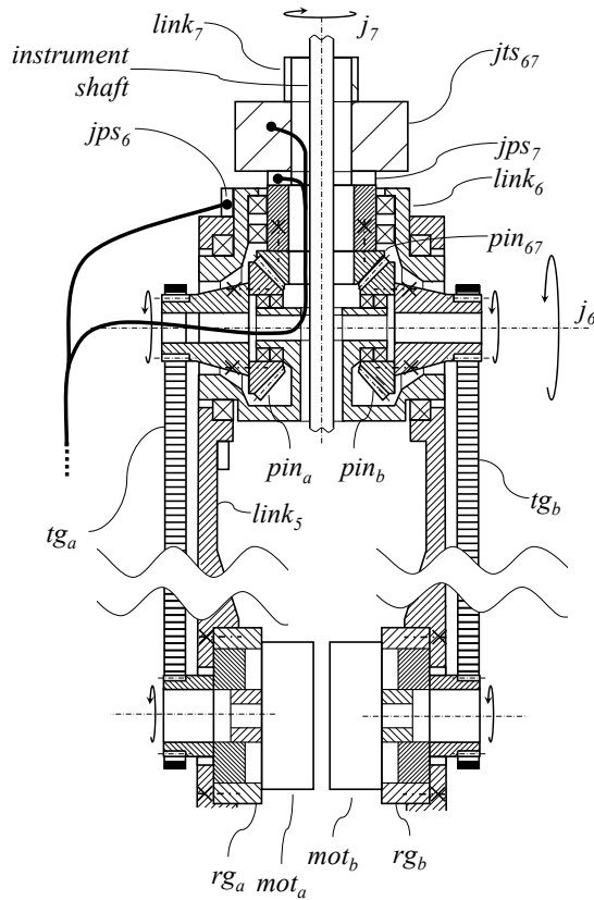
Figure 4.33: The miro_{67} design concept (1)
