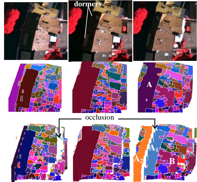
Figure 1. Upper row: original images; two dormers are indicated in one image. Second row: results of watershed segmentation using k = 2 and N_s = 5 . Last row: segmentation results projected to object space. Two areas where occlusions occurred are marked.
