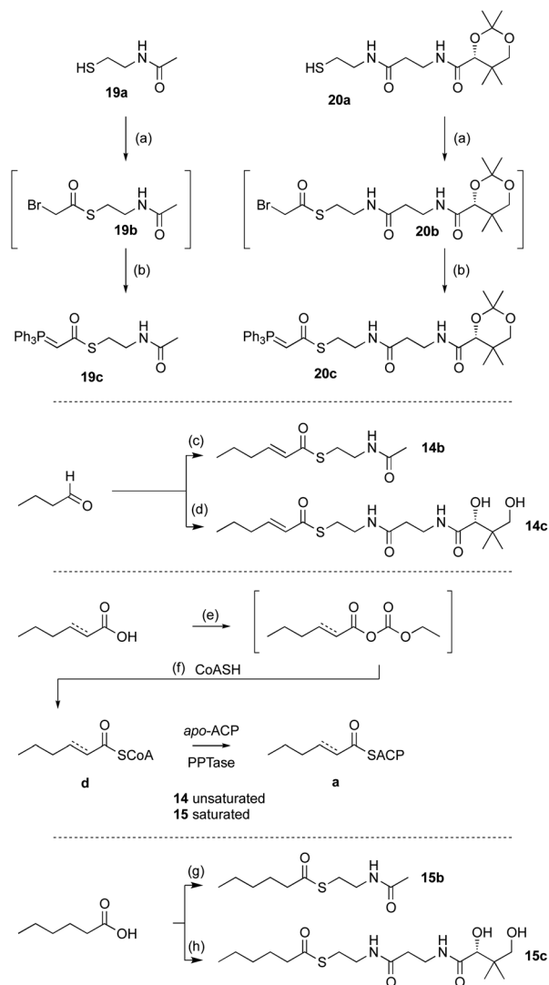
Scheme 2 Synthesis of hex(en)oyl substrates. Reagents and conditions: (a) BrCH 2 CO 2 H, EDCl, DMAP, CH 2 Cl 2 , RT; (b) PPh 3 , toluene, 80 °C, then aq. NaOH; (c) 19c , CH 2 Cl 2 , RT, 72 h; (d) 20c , CH 2 Cl 2 , 40 °C, 3 d then THF/CF 3 CO 2 H, RT, 60 min; (e) ClCO 2 Et, CH 2 Cl 2 , Et 3 N, 0 °C; (f) CoASH, aq. NaHCO 3 ; (g) 19a , EDCl, DMAP, CH 2 Cl 2 ; (h) 20a , EDCl, DMAP, CH 2 Cl 2 , then THF/CF 3 CO 2 H, RT, 60 min.
