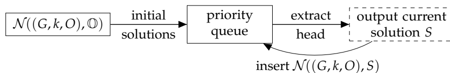
Figure 1. Structure of Algorithm 2.
