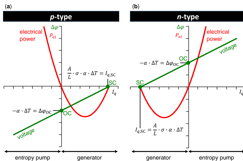
Figure A1. Voltage \Delta\varphi – electrical current I_q characteristics (green curves) and electrical power P_{\text{el}} – electrical current characteristics I_q (red curves) for materials with: (a) Seebeck coefficient \alpha being positive, which refers to p -type conduction and (b) Seebeck coefficient \alpha being negative, which refers to n -type conduction. Here, \Delta T = \frac{T_{\text{hot}} - T_{\text{cold}}}{T_{\text{hot}}} is the temperature difference along a thermoelectric material of length L and cross-sectional area A . These quantities, together with the (isothermal) electrical conductivity \sigma and the Seebeck coefficient, determine the electrical current I_{\text{SC}} under electrical short-circuited conditions. The voltage \Delta\varphi_{\text{OC}} under electrical short-circuited conditions is determined by the Seebeck coefficient and the temperature difference. When the electrical power P_{\text{el}} is negative (electrical power output), the material is in generator mode (thermal-to-electrical power conversion). When the electrical power P_{\text{el}} is positive (electrical power input), the material is in entropy pump mode (electrical-to-thermal power conversion).
