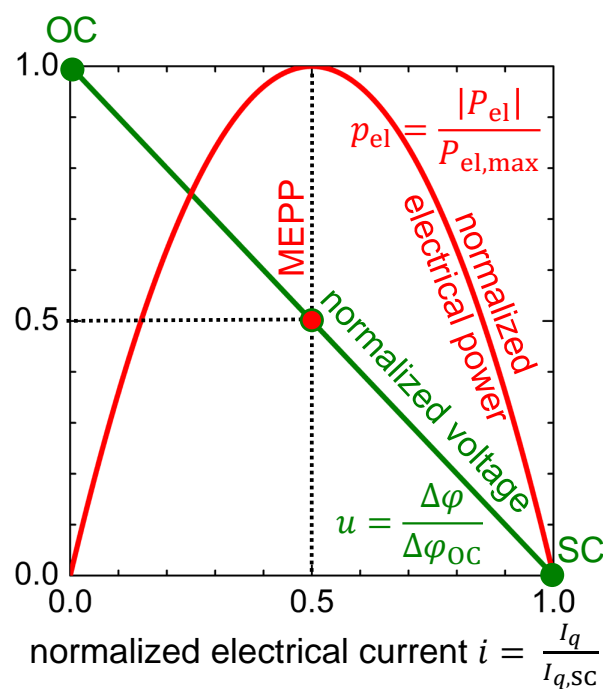
Figure 4. Normalized curves for both voltage u – electrical current i characteristics and electrical power p_{el} – electrical current i characteristics of a thermoelectric material when it is operated in generator mode. The working points open-circuited (OC), maximum electrical power point (MEPP), and short-circuited (SC) are indicated.
