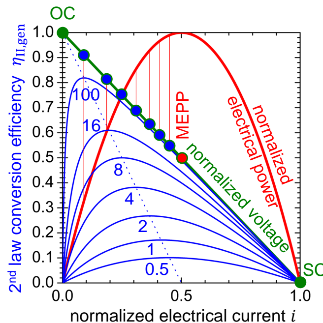
Figure 6. Thermal to electrical power conversion efficiency for some hypothetic materials with figure-of-merit zT varying from 0.5 to 100. Respective working points MCEP (blue) are indicated on the voltage–electrical current curve as well as the MEPP (red). Vertical lines indicate the electrical power output at the MCEP for the example materials. Note that the MCEP drifts apart from the MEPP with increasing figure-of-merit zT . The dashed line indicates the dependence of the MCEP with varying zT .
