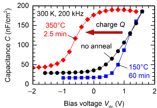
FIG. 3. Fixed interface-charge formation. Capacitance-voltage characteristics C(V_{\text{dc}}) at T = 300 K and f = 200 kHz of a \text{Au}/\text{Al}_2\text{O}_3/\text{CIGS} M-I-S device with 20 nm \text{Al}_2\text{O}_3 after different annealing procedures in nitrogen ambient: no annealing (black circles), 60 min at 150^\circ\text{C} (blue squares), and 2.5 min at 350^\circ\text{C} (red diamonds).
