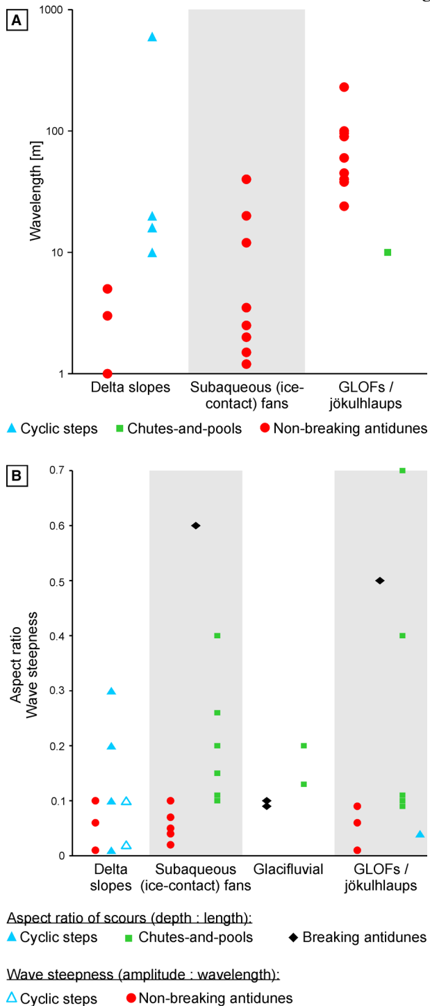
Fig. 12. Upper-flow-regime bedform dimensions measured in different glacigenic depositional environments. (A) Wavelengths of different bedform types. (B) Aspect ratios and wave steepness of different bedform types (GLOF, glacial lake-outburst flood).
