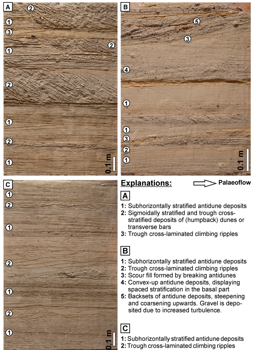
Fig. 4. Photographs of lacquer peels of upper-flow-regime bedforms in glacial fluvial deposits (Werpeloh, northern Germany; Middle Pleistocene). The palaeoflow direction is approximately from the left in all peels.
