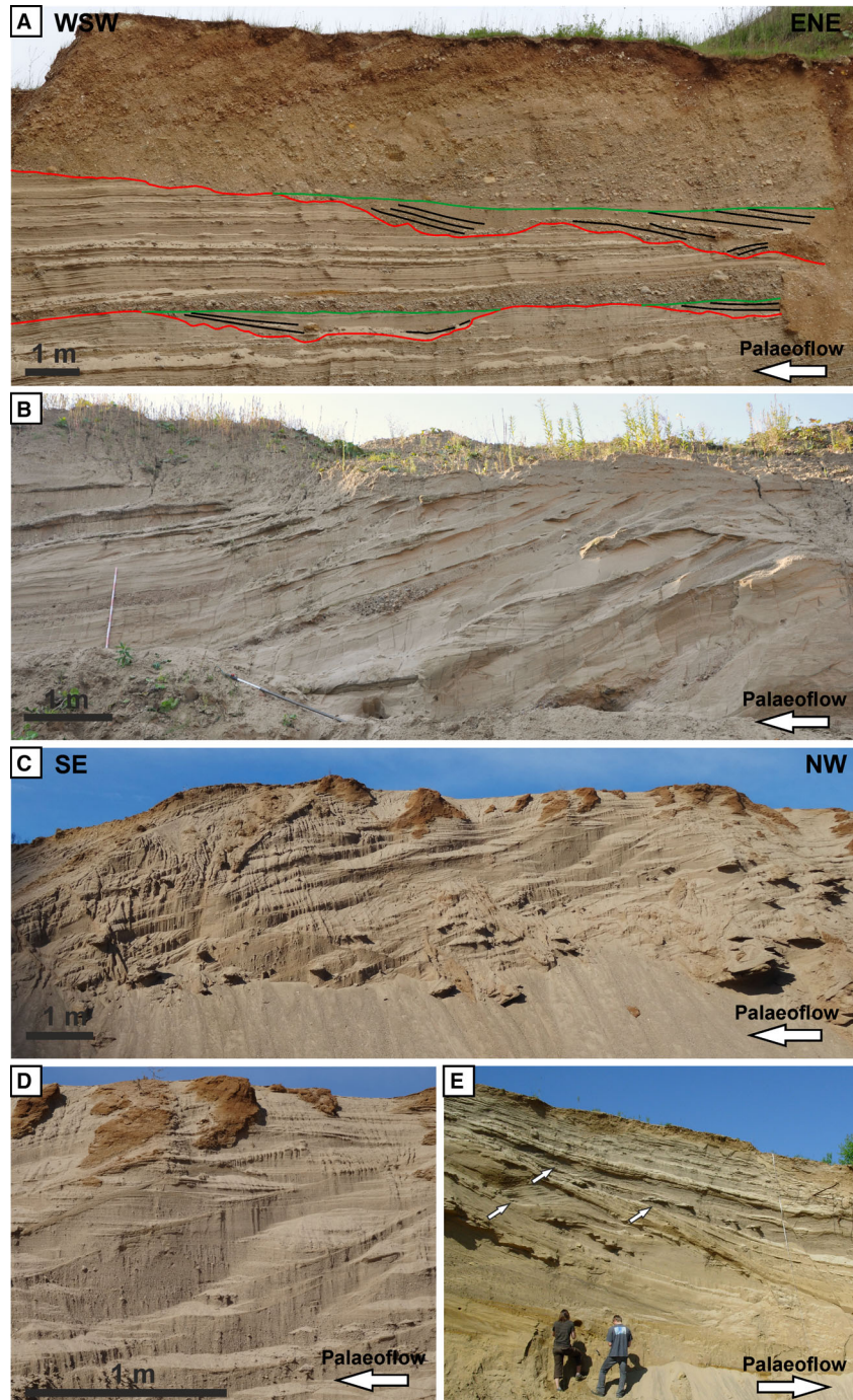
Fig. 9. Upper-flow-regime bedforms in glacial fluvial deltas. (A) Deposits of cyclic steps overlie erosional surfaces (red) formed during forced regression. Cyclic-step deposits comprise elongate scours filled by backsets. Prograding delta-foreset deposits downlap the erosional surfaces and cyclic-step deposits (Betheln Delta, northern Germany; Middle Pleistocene; modified from Kostic et al. , 2019). (B) Delta-foreset deposits, comprising, isolated gravelly and sandy backset cross-stratified scour fills, which are interbedded with sinusoidally stratified sand. The succession is interpreted as deposits of cyclic steps and superimposed antidunes that were formed by surge-type supercritical density flows. Tool for scale is 1.4 m (Porta Delta, northern Germany; Middle Pleistocene). (C) Delta-foreset deposits, comprising laterally stacked scours filled by backset cross-stratified pebbly sand interpreted as cyclic steps deposited by sustained supercritical density flows (Freden Delta; northern Germany; Middle Pleistocene). (D) Detail of the stacked backset cross-stratified scour fills from Fig. 5C. (E) Isolated backset cross-stratified scour-fills (arrows) related to cyclic steps within foreset packages dominated by climbing-ripple cross-laminated sand (Freden Delta, photograph by courtesy of C. Brandes; modified from Lang et al. , 2017b, and Winsemann et al. , 2018).
