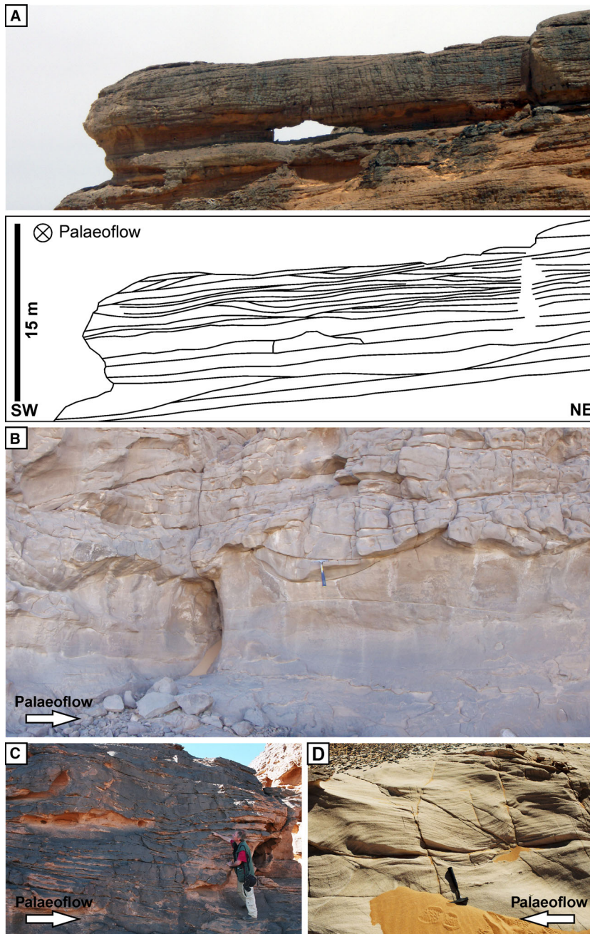
Fig. 11. Upper-flow-regime bedforms deposited by supercritical density flows in glacialmarine settings (North Africa; Upper Ordovician). (A) Sheet-like sandstones that display sinusoidal stratification and low-angle cross-stratification with common internal low-angle truncations, pointing to deposition by antidunes (Jebel Asba region, Kufra Basin, Libya). (B) Thickly bedded sinusoidally stratified sandstone, indicating highly aggrading antidune deposits, is unconformably overlain by foreset and backset cross-stratified sandstone, probably indicating chutes-and-pools. Hammer for scale is 33 cm (Jebel Eghei region, Kufra Basin, Libya; from Le Heron et al. , 2014). (C) Sinusoidally stratified sandstone deposited by antidunes (Tassili N'Ajjer region, Illizi Basin, Algeria). (D) Sigmoidally stratified sandstone deposited by humpback dunes, passing upward into sinusoidally stratified antidune deposits. Hammer for scale is 33 cm (Jebel Asba region, Kufra Basin, Libya; from Le Heron et al. , 2010).
