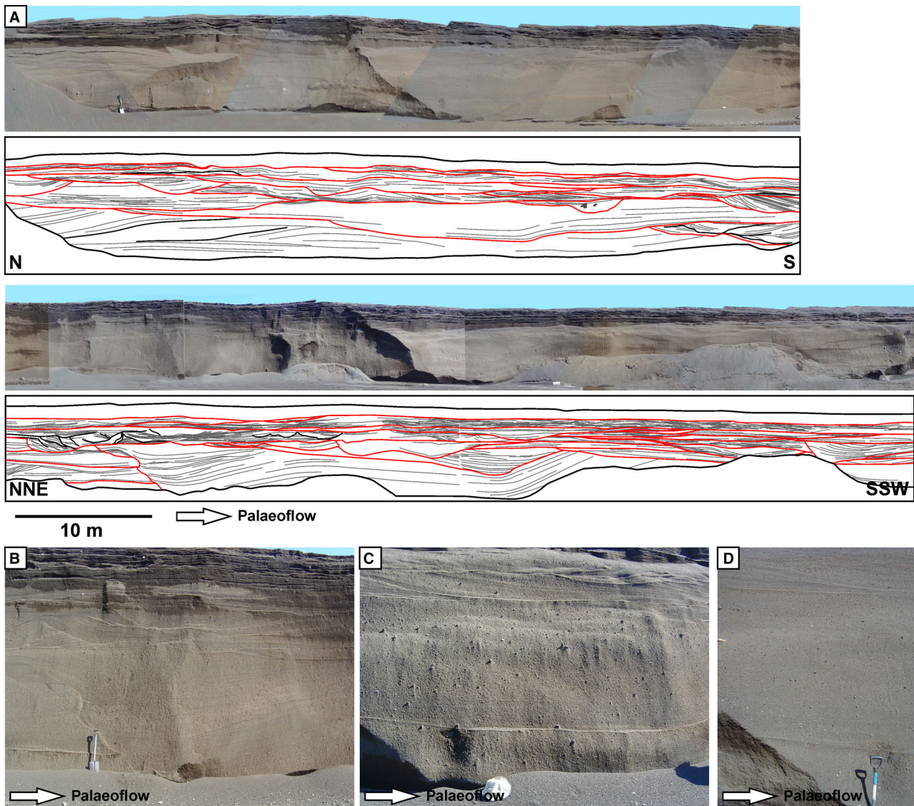
Fig. 6. Upper-flow-regime bedforms formed during a jökulhlaup (Mýrdalssandur, Iceland; Holocene). All photographs by courtesy of R. Duller. (A) Interpreted ‘photo panel’ of the jökulhlaup deposits. The succession comprises laterally and vertically stacked deposits of antidunes and chutes-and-pools (modified from Duller et al. , 2008). (B) Detail of a steep-walled scour margin interpreted as chute-and-pool deposit. Shovel for scale is ca 1 m. (C) Detail of the antidune deposits. The diffusely stratified to almost structureless sediment relates to the homogeneity of the scoria gravel and the rapid sedimentation from concentrated flows. Hat for scale is ca 45 cm (modified from Duller et al. , 2008). (D) Detail of the antidune deposits, showing an almost structureless ca. 1.5 m thick bed. Shovel handle for scale is ca 75 cm.
