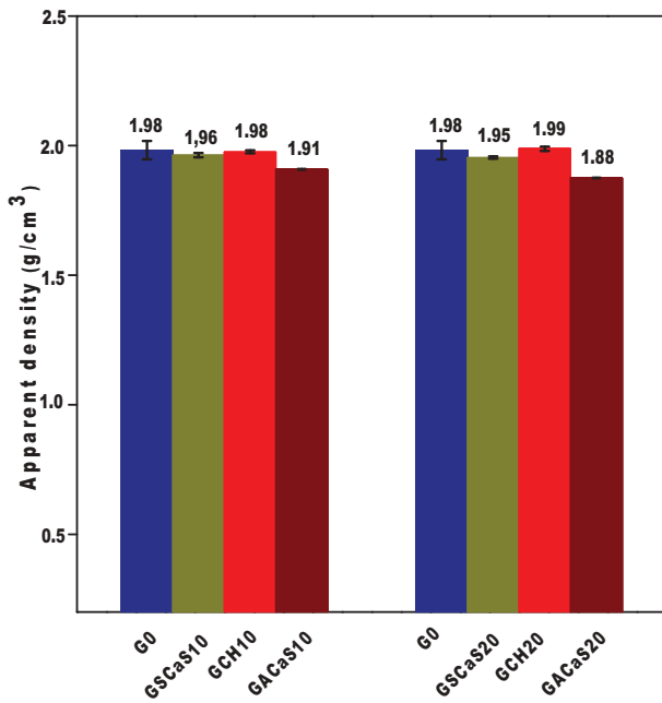
Figure 8. Apparent density of metakaolin-based geopolymer cements.
