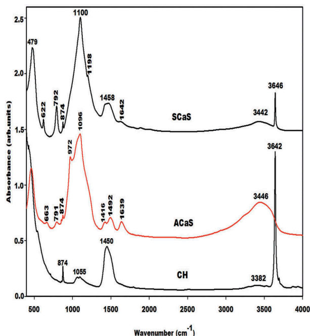
Figure 3. Infrared spectra of calcium hydroxide (CH), nanocomposite (ACaS) and microcomposite (SCaS).
