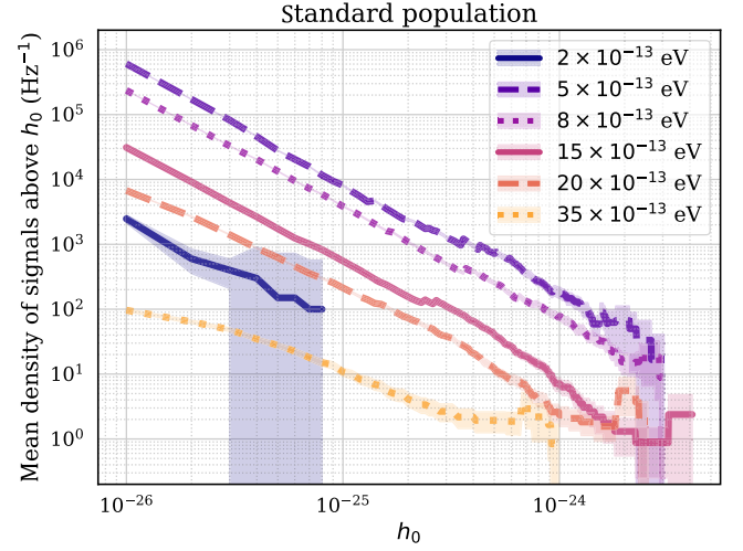
FIG. 16. The mean density of signals above a given h_0 . The mean density is largest for \mu_b = 5 \times 10^{-13} eV ( f_{\text{GW}} \approx 250 Hz) for the standard black hole population (Table I). For heavier bosons, the overall density decreases; the number of signals above a given h_0 drops due to the combination of effects described in Fig. 15, while the frequency range spanned by the ensemble signal continues to increase. The contours show the uncertainty \sqrt{N}/\Delta f , where N is the number of signals and \Delta f is the frequency range spanned by the N signals. Note that this does not take into account the additional uncertainty from \Delta f , which is itself correlated with N .
