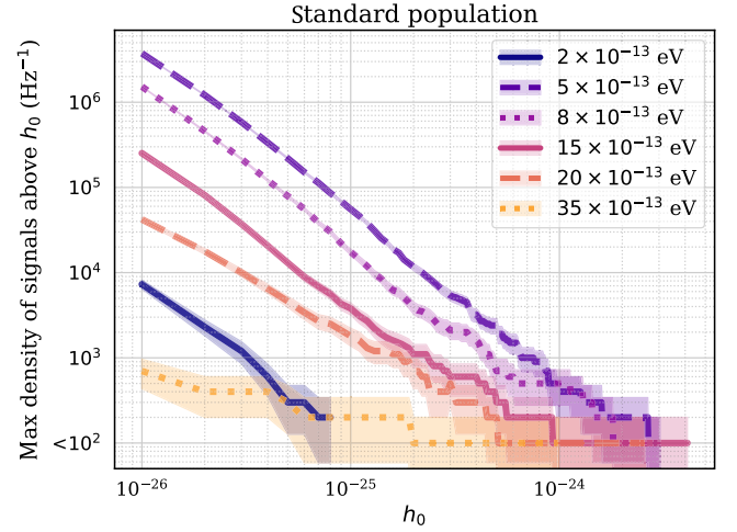
FIG. 17. The maximum density of signals above a given h_0 is up to an order of magnitude larger than the mean density (Fig. 16). Frequency ranges with sufficiently high signal densities can cause complications for standard searches for continuous wave signals (Sec. V). The contours show the uncertainty \sqrt{N}/\Delta f , where N is the number of signals and \Delta f = 0.01 Hz is the size of the frequency bin over which the maximum density is calculated.
