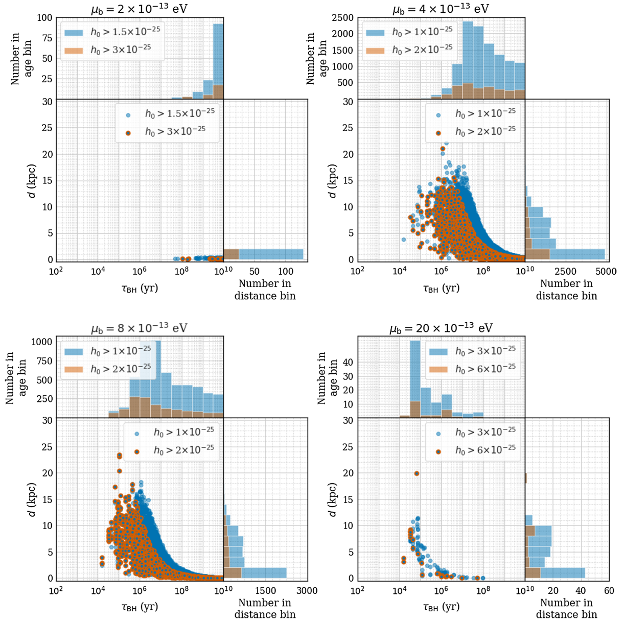
FIG. 34. Ages and distances of the heavy black hole population. As in Fig. 33, the addition of black holes with M_{\text{BH}} > 20M_{\odot} increases the number of detectable systems for the lighter bosons ( \mu_b = 2 \times 10^{-13} and 4 \times 10^{-13} eV) but has little to no effect on the heavier bosons.
