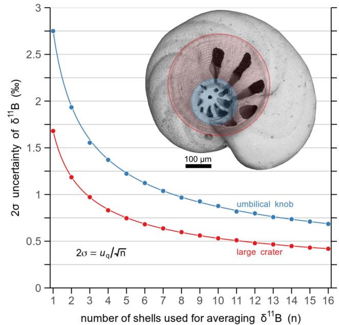
Figure 7. Results from Monte Carlo simulations of 2\sigma uncertainty for \delta^{11}\text{B} using LA-MC-ICPMS in relation to the number of analyzed C. wuellerstorfi shells ( n ). In red is the estimated uncertainty based on “large crater”, and in blue on “umbilical knob” measurements (see inset scanning electron microscope picture for different areas). The estimated 2\sigma uncertainty can be described by a function of the quoted uncertainty ( u_q ) and n (Eq. 3).
