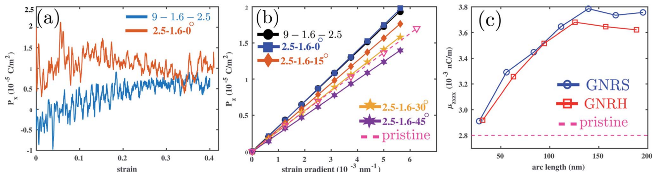
Fig. 5 (a) Variation of polarization P_x with tensile strain. (b) Bending induced polarization P_z response with respect to the strain gradient. (c) Dependence of the flexoelectric coefficient \mu_{zzxx} on the arc length of GNRS and GNRH systems. Legends indicate the respective atomic configurations used.
