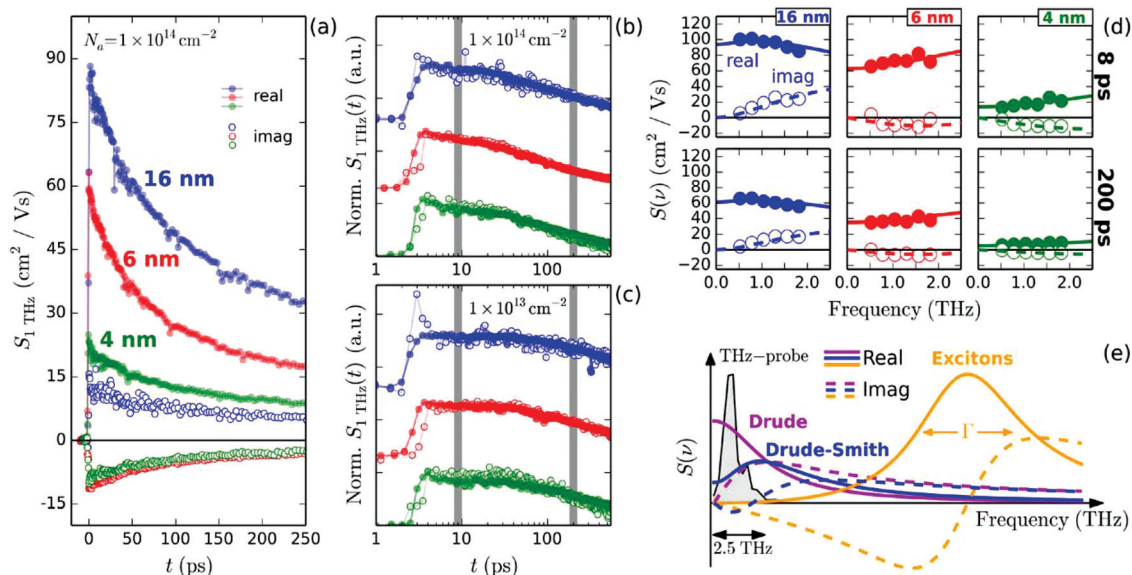
Fig. 2 (a) Decay-kinetics of the real (filled circles) and imaginary (open circles) component of the transient THz signal S(\nu = 1 \text{ THz}) for 16 (blue), 6 (red) and 4 nm (green) PbS-NSSs. N_a indicates the number of absorbed photons per \text{cm}^2 (see text). (b and c) Comparison between the normalized S_{\text{Re}} and S_{\text{Im}} at high and low N_a , exhibiting the same decay kinetics (d) Transient frequency-dependent THz signals obtained at 8 ps (upper panels) and 200 ps (lower panels) after excitation [gray vertical lines in (b) and (c)] at N_a \sim 5 \times 10^{13} \text{ cm}^{-2} . Solid and dashed lines are fits of the real and imaginary components obtained from eqn (2)–(4). (e) Scheme of the response of free charge carriers without backscattering [magenta, eqn (3) with c = 0 ], with backscattering [blue, eqn (3) with c = -1 ] and EXs [orange, eqn (4)].
