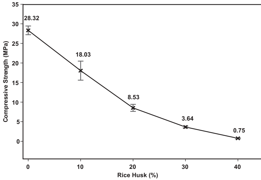
Figure 10. Compressive strengths of geopolymer mortars as function of replacement level of metakaolin by rice husk.
