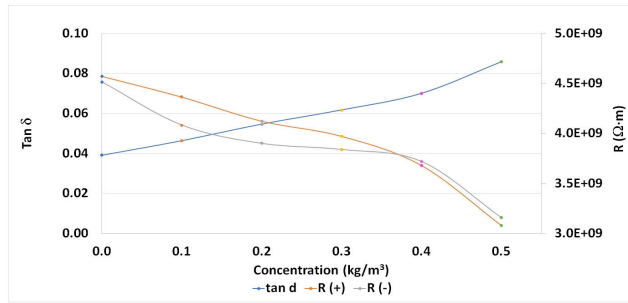
FIGURE 9. Dissipation factor and resistivity of tested samples.
