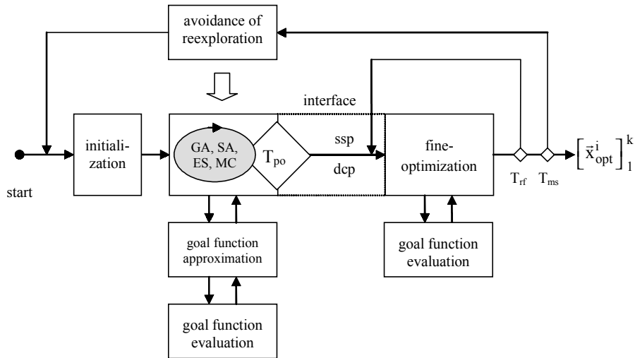
Figure 11. Application of different pre-optimization strategies in cyclical change
