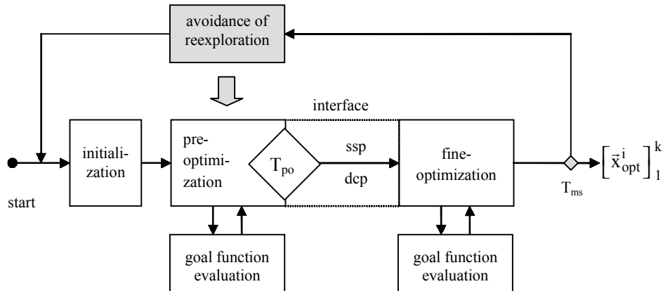
Figure 7. Basic structure of a multiple-stage optimization strategy
