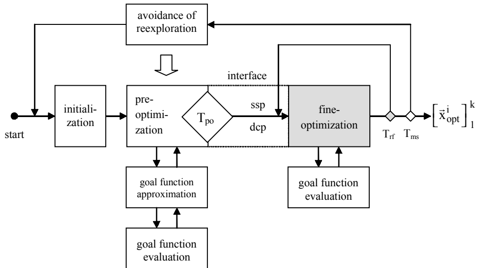
Figure 9. Repeated start of fine-optimization
