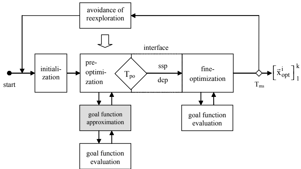
Figure 8. Acceleration of pre-optimization through goal function approximation
