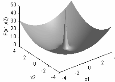
Figure 10. Misleading problem for evolutionary algorithms
