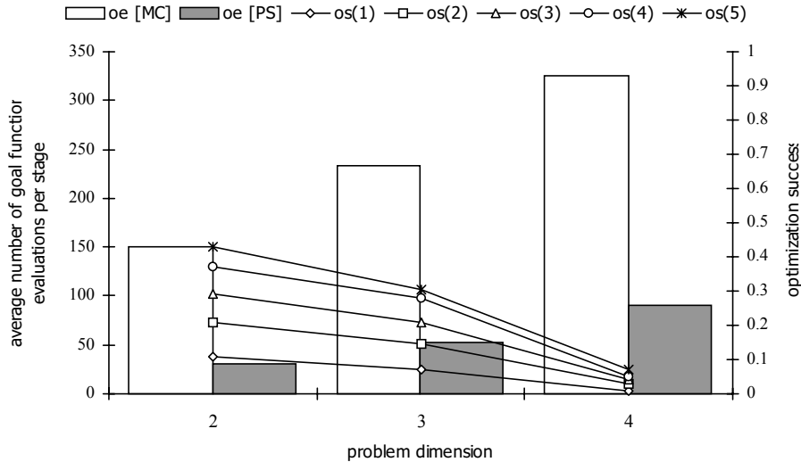
Diagram 2. Results of optimization experiment E_2
