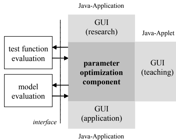
Figure 13. Graphical user interface (GUI) of the optimization component
