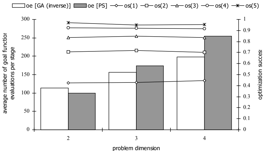
Diagram 3. Results of optimization experiment E_3
