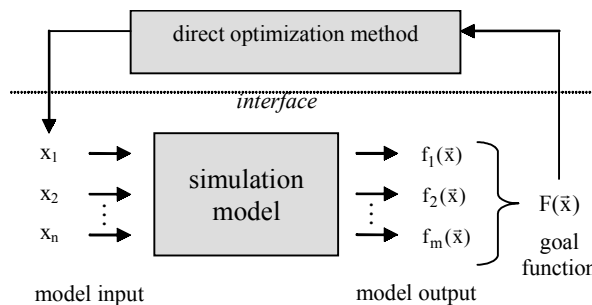
Figure 5. Parameter optimization of a simulation-based goal function
