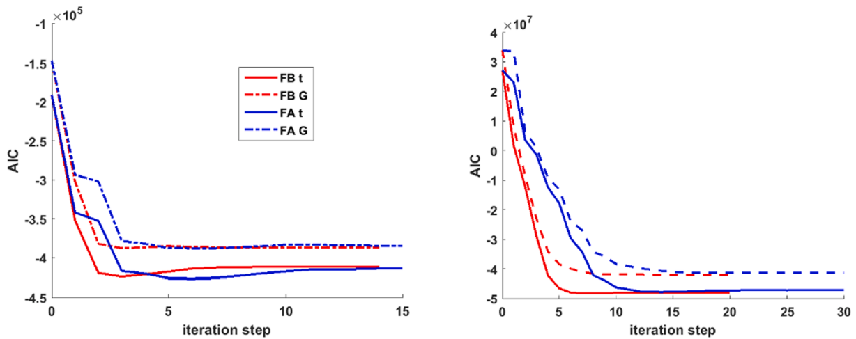
Fig. 3. Left: FA_AIC and FB_AIC with respect to the number of iterations for the two distributions (normal G: dotted line and t for the t-distribution: full line) for the small dataset. The first iteration step is labelled as 0. Right: same as left for the whole dataset.
