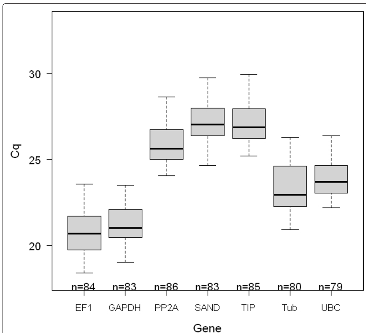
Figure 1 The expression levels of the reference candidates over all treatments. The boxplot graphs show the measured quantification cycles (Cq) for all candidate genes comprising all genotypes (93/1-119, 94/1-30 and 94/1-97), all tissues (leaves, roots and immature flower buds) and all treatments (heat shock, wounding, black spot inoculation for 2 h and 3 d) of genotype 93/1-119. The boxes represent 25 and 75 quartiles, the whisker caps indicate 10 and 90 percentiles, and the medians are indicated by the line. The number of included Cqs is indicated by n.
