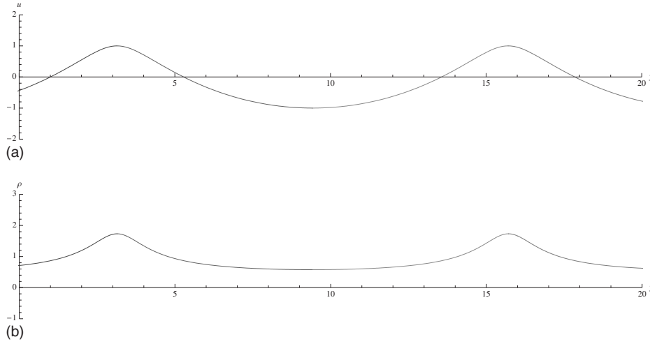
FIG. 1. A traveling-wave solution (u, \rho) of the two-component HS equation (1.4) with \sigma=1 and the parameter values b=1 , z=-1 , Z=1 , c=2 . The top and bottom graphs show u and \rho as functions of y=x-ct , respectively.
