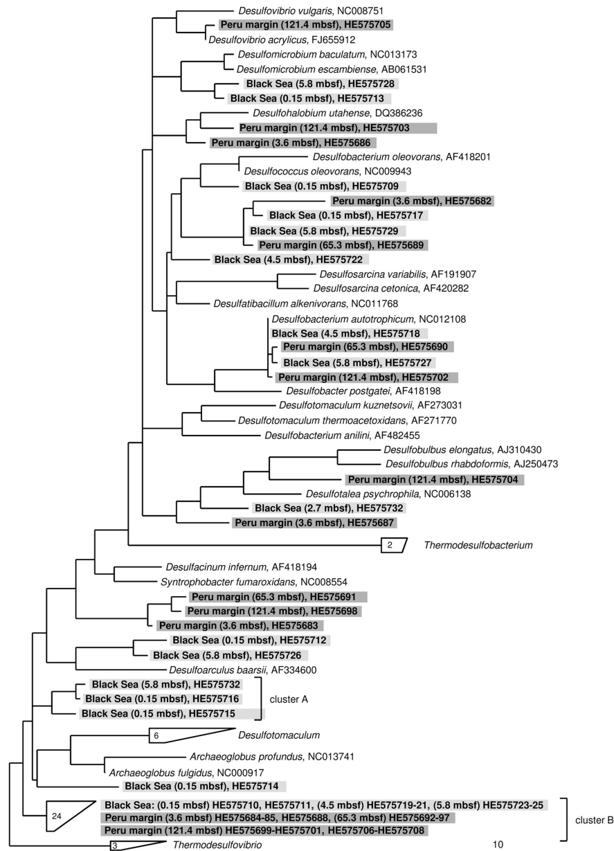
FIGURE 3 | Gene dsrA phylogeny based on deduced amino acid sequences of the dsrA gene coding for the alpha subunit of dissimilatory (bi)sulfite reductase. Sequences from
