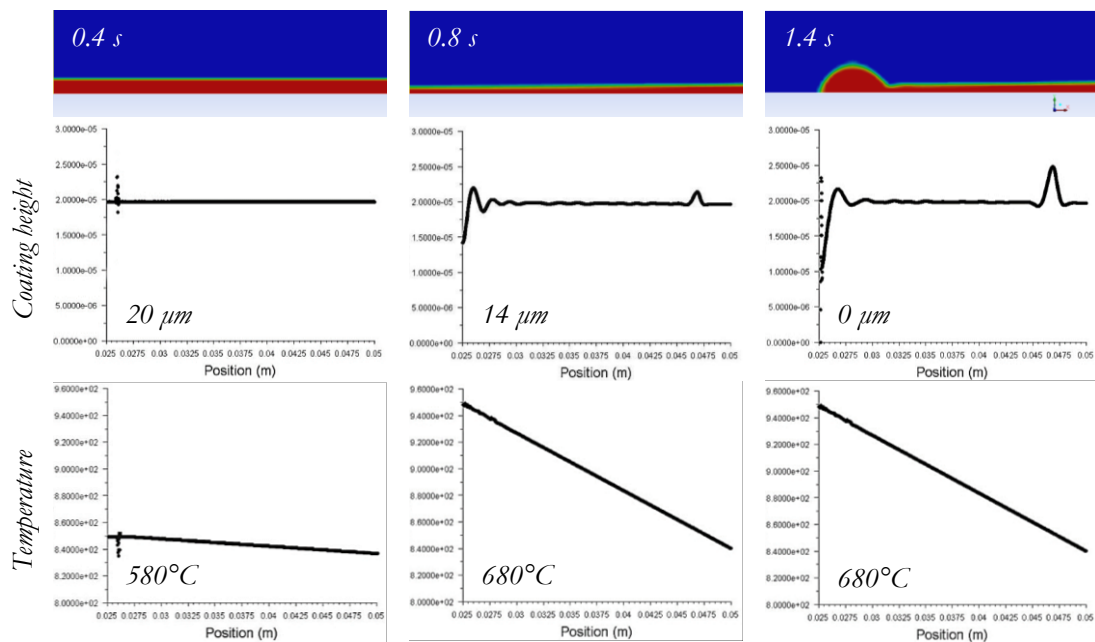
Figure 5. 2D-VOF-simulation sequence from coating melting ( t=0.4s ) over dryspot formation ( t=0.8 ) till wave propagation ( t=1.4s ) based on a triangle temperature profile and resulting Marangoni forces by applying a temperature gradient of 70\text{ }^{\circ}\text{C} over a measuring length of 50\text{ mm} .
