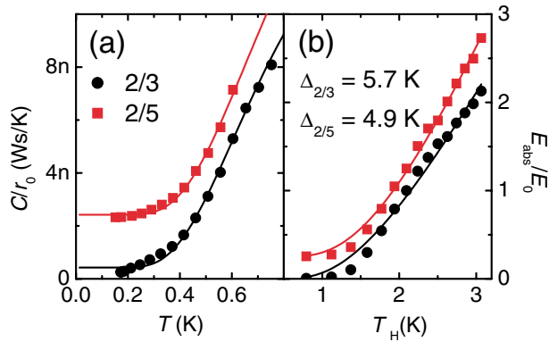
FIG. 2 (color online). (a) Examples of the relative specific heat at filling factors \nu = 2/3 and 2/5 measured by phonon absorption for sample #5 ( n = 1.21 \times 10^{15} \text{ m}^{-2} ). Data for 2/5 are shifted for clarity by 2n . The lines are fits according to Ref. [14] plus a constant. (b) Relative phonon energy absorbed by the 2DES, normalized to its value E_0 for T_H = 2.09 \text{ K} , for a 10-ns pulse at filling factors \nu = 2/3 and 2/5 (data for 2/5 are shifted by 0.25 for clarity). The curves are fits for an excitation across a gap \Delta_{2/3} = 5.7 \text{ K} and \Delta_{2/5} = 4.9 \text{ K} .
