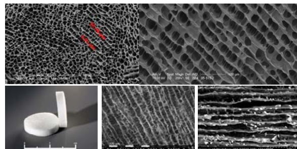
Figure 1: Pictures of structures made by ice templating.
