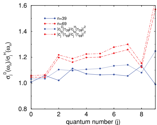
FIG. 5. (Color online) Ratio of harmonic signals from D_2O and H_2O as a function of the quantum number of the initial vibrational state in the neutral molecule. Shown are the ratios of integrated harmonic peaks for two different harmonic orders n (solid blue and dashed red curves) as well as the corresponding ratios expected from the autocorrelation function (dotted blue and dot-dashed red curves).
