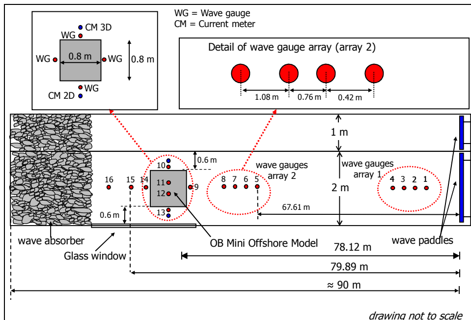
Figure 2. Model set-up in the 2m-wide wave flume at LWI (plan view)
