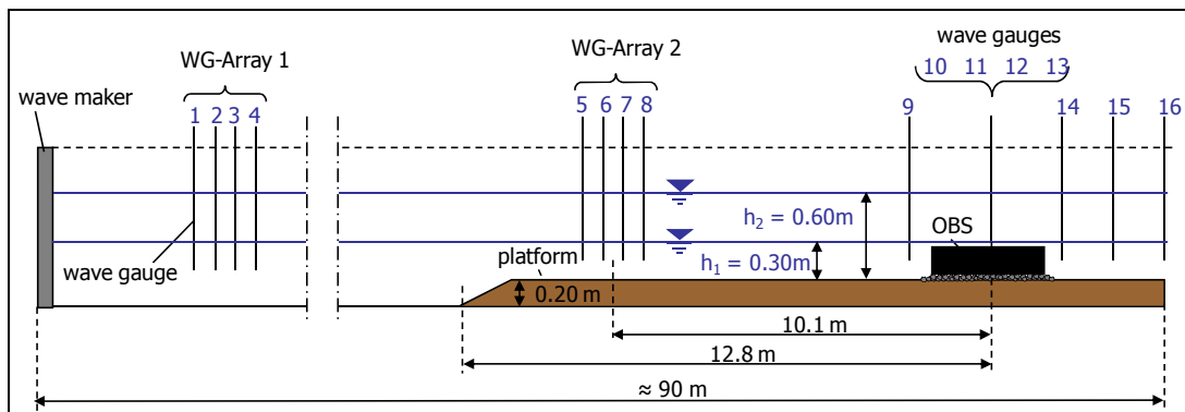
Figure 3. Position of the wave gauges and the OBS-model in the wave flume (cross section)
