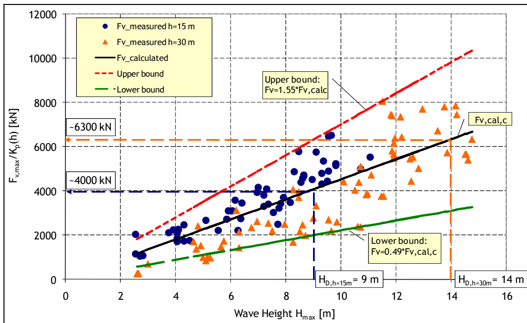
Figure 9. Comparison of calculated and measured vertical wave forces (prototype scale)
