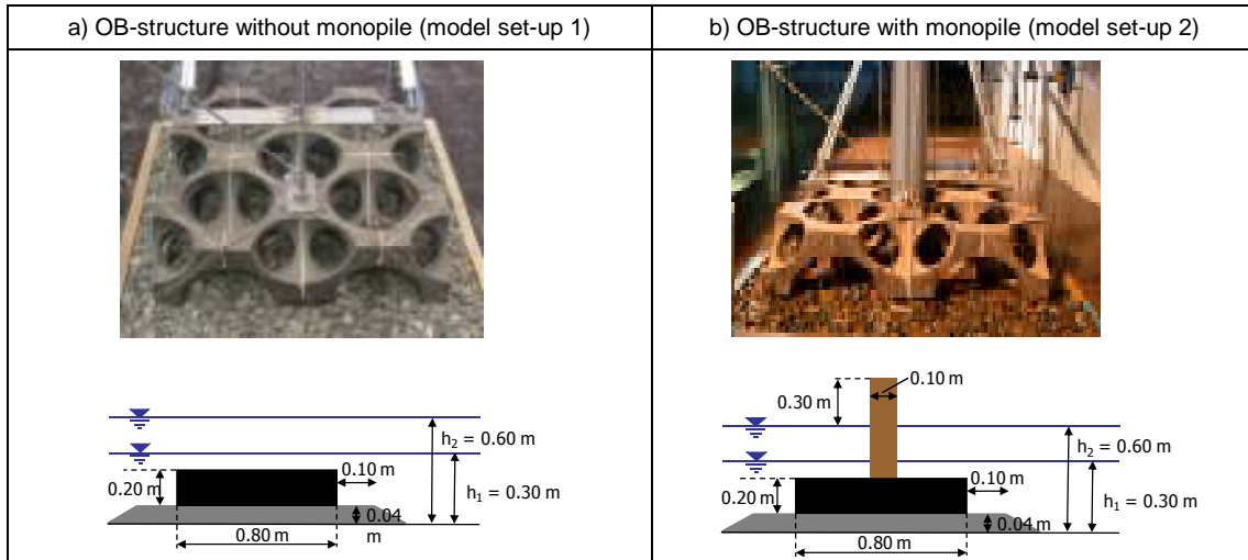
Figure 1. OBS used as a foundation structure for offshore wind turbine (model scale 1:50)
