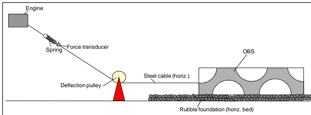
Figure 11. Sliding tests for the determination of the friction coefficient
