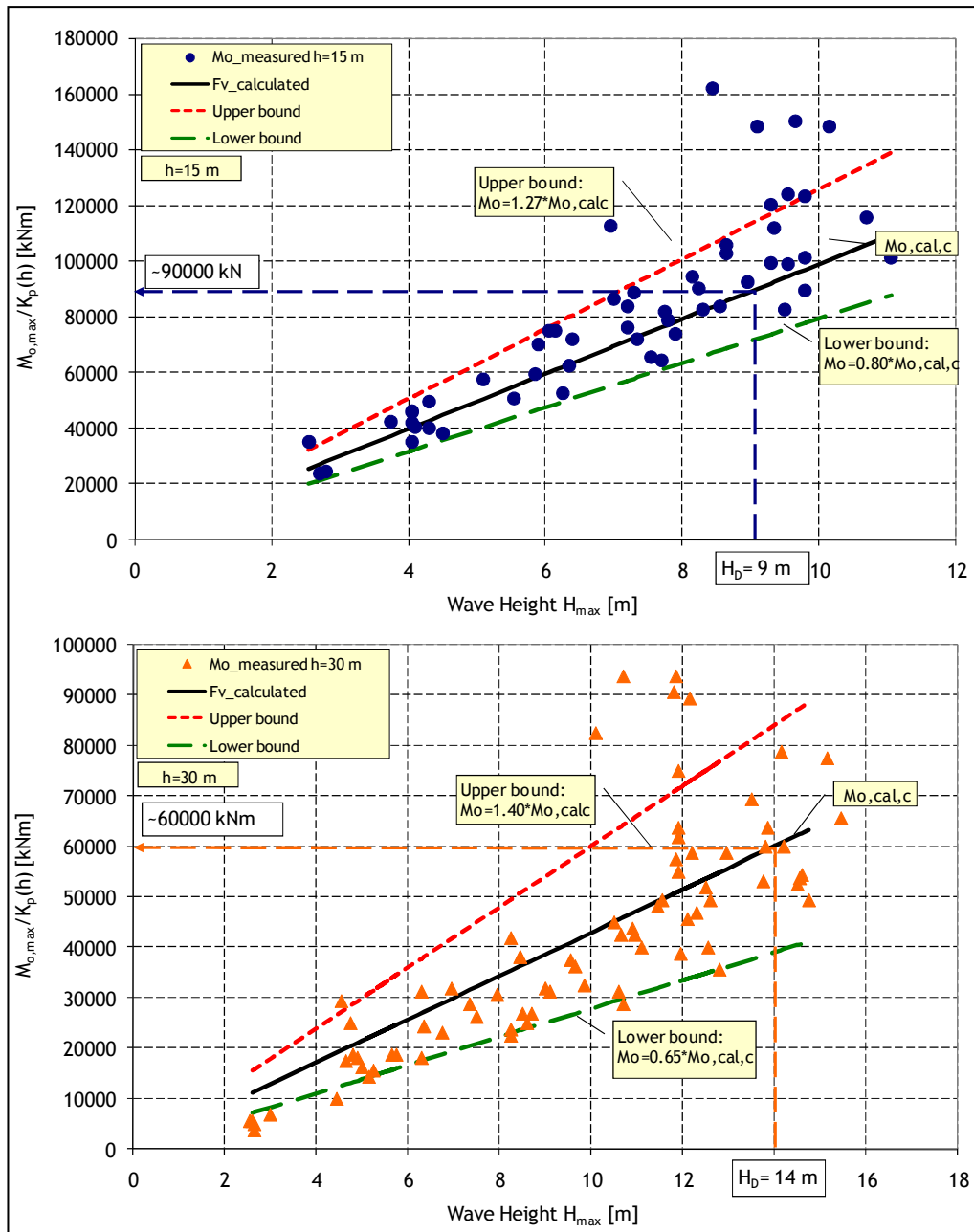
Figure 10. Comparison of calculated and measured overturning moments (prototype scale)
