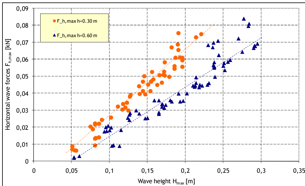
Figure 5. Measured maximum horizontal wave forces on the OBS-model without monopile (see Fig. 1a)
