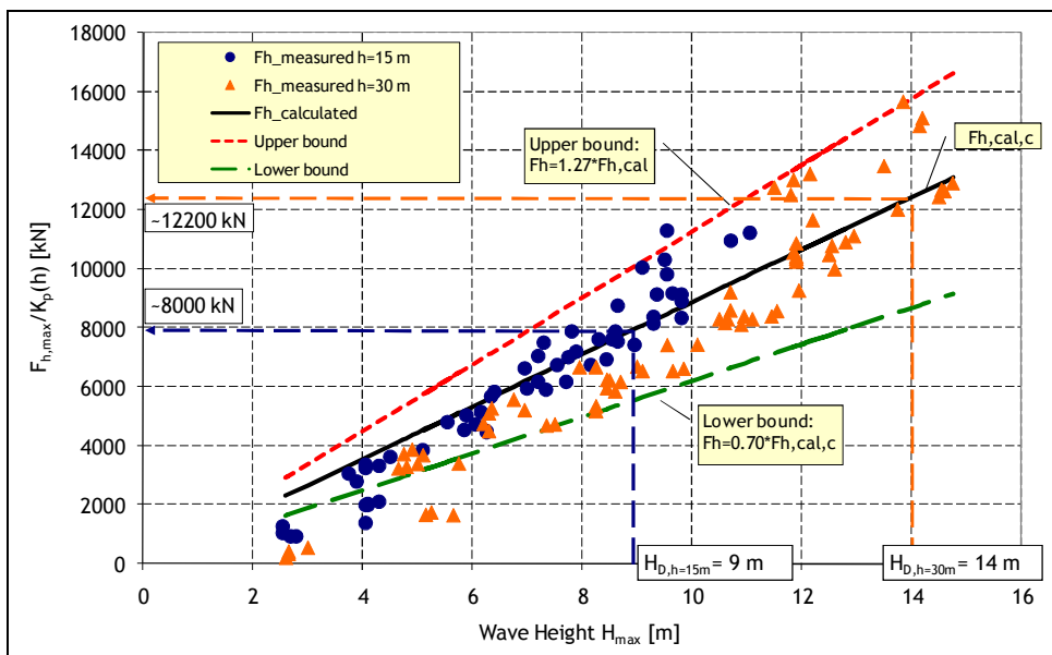
Figure 7. Comparison of calculated and measured horizontal wave forces (prototype scale)
