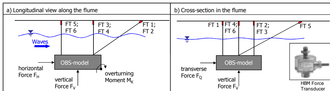
Figure 4. Total wave load transducer and OBS model
