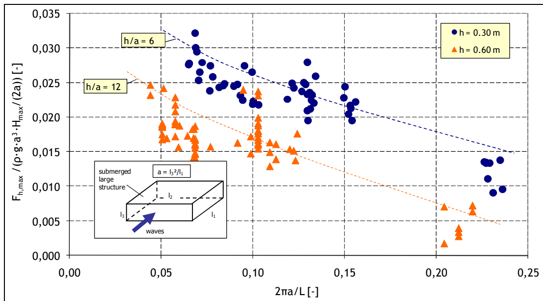
Figure 8. Effect of diffraction parameter 2\pi a/L and relative water depth h/a on dimensionless horizontal wave force
