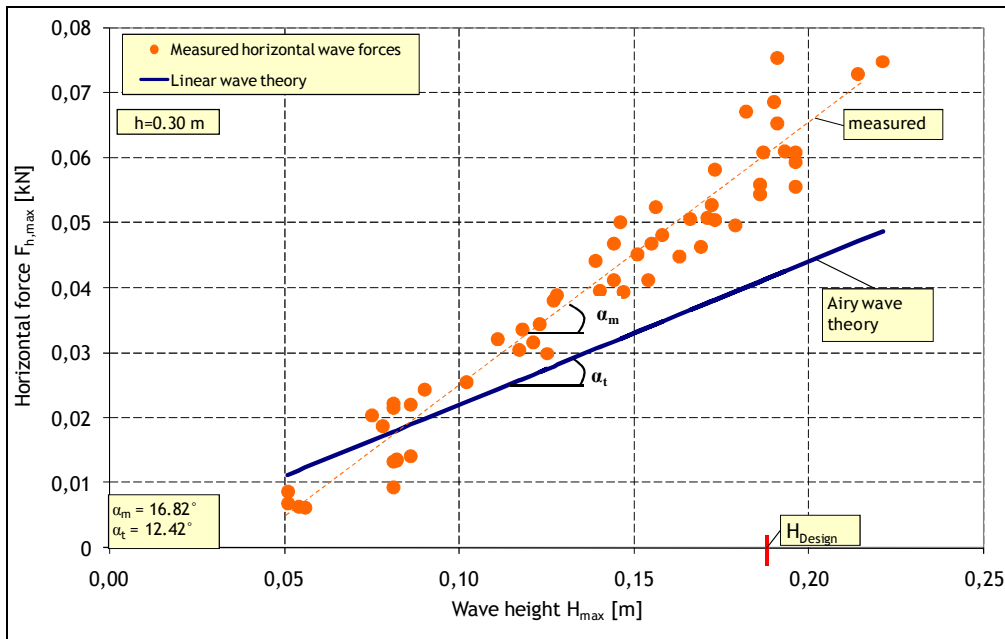
Figure 6. Comparison of measured and calculated wave forces for water depth h=0.30\text{m}
