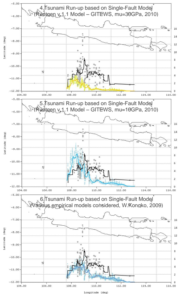
Figure 9. Model validation of run-up (source 4-6)
