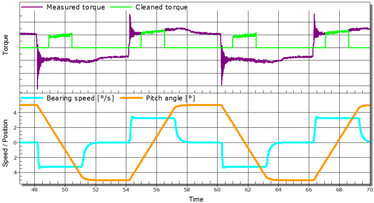
Figure 3: Oscillating movements and torque measurements (example)
