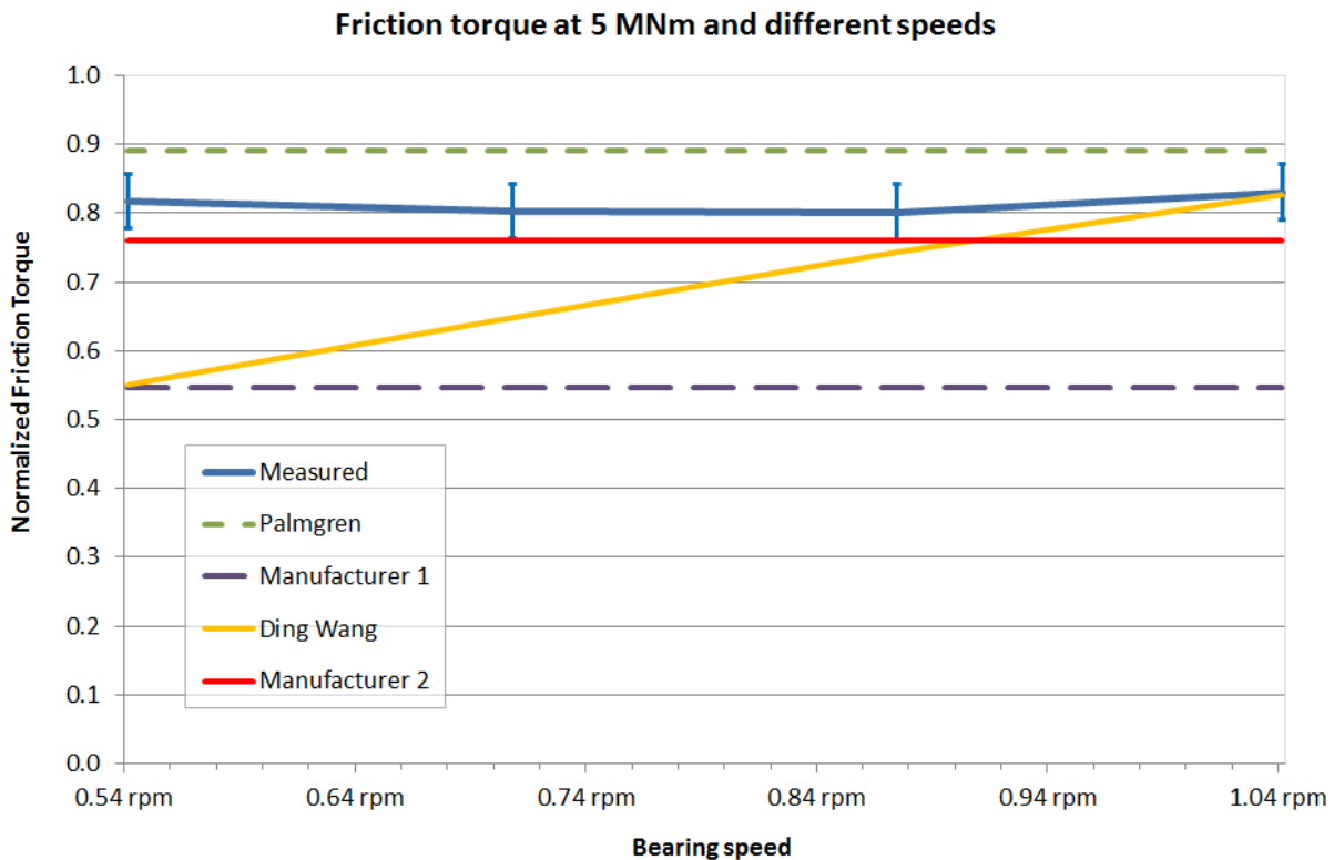
10 Figure 8: Measured and calculated friction torque at different speeds and 5 MNm load
