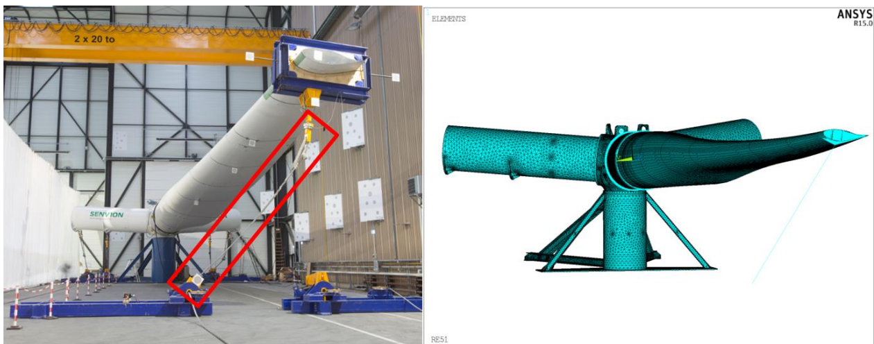
10 Figure 1: Pitch bearing test rig at Fraunhofer IWES and corresponding FE model.
