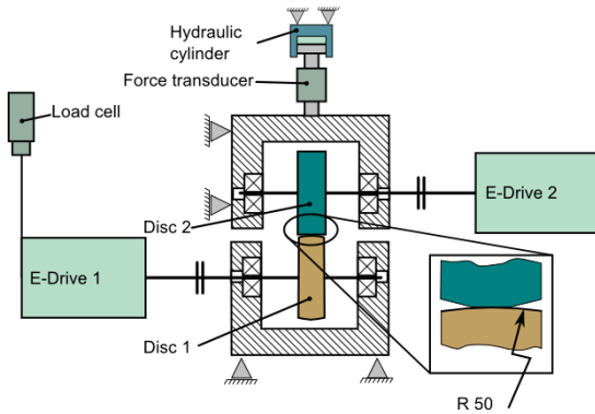
Figure 4: Two disc machine
