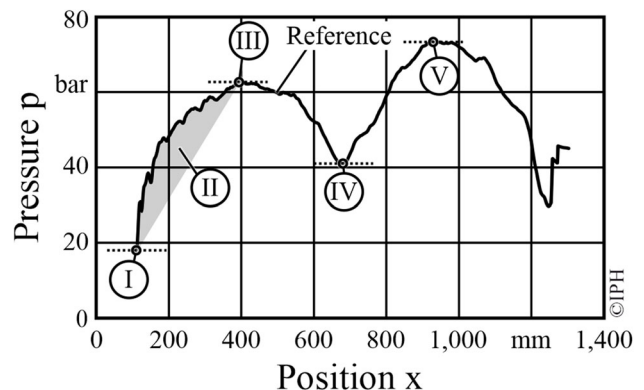
Fig. 8 Pressure curve of CWR with characteristic points
