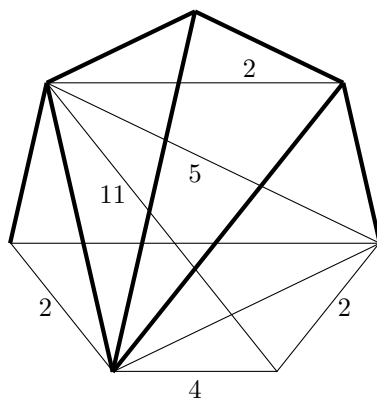
FIGURE 11. Third step of the extension of \mathcal{C} .
