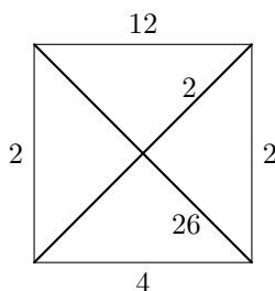
FIGURE 8. A frieze with coefficients on a square.
