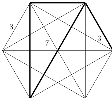
FIGURE 10. Second step of the extension of \mathcal{C} .
