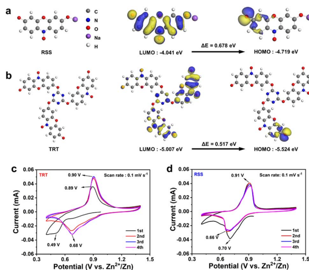
Fig. 2 Theoretical simulations of RSS and TRT. Calculated HOMO and LUMO of (a) RSS and (b) TRT. CV curves of (c) TRT and (d) RSS under 0.1 mV s -1 .
