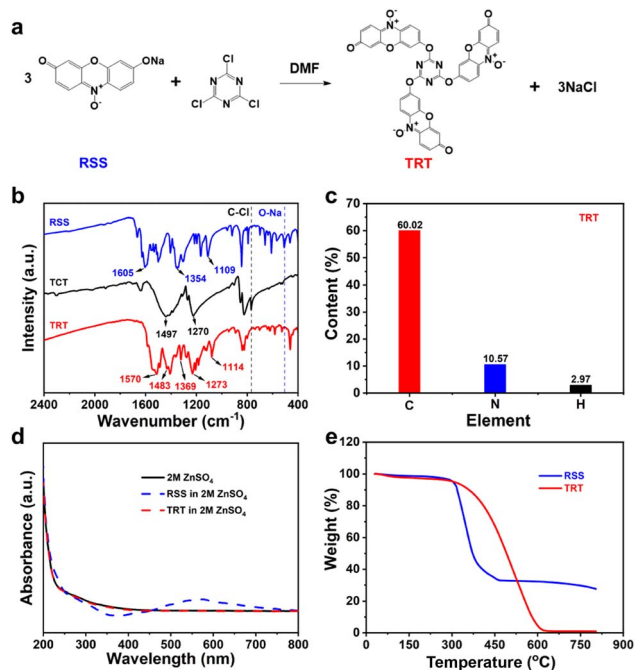
Fig. 1 (a) Synthesis procedure of TRT. (b) FT-IR spectra of RSS, TCT, and TRT. (c) Elemental analysis result of TRT. (d) The comparison of UV-vis spectra of RSS and TRT in the electrolyte (2 M ZnSO 4 ). (e) Thermogravimetric analysis of RSS and TRT.
